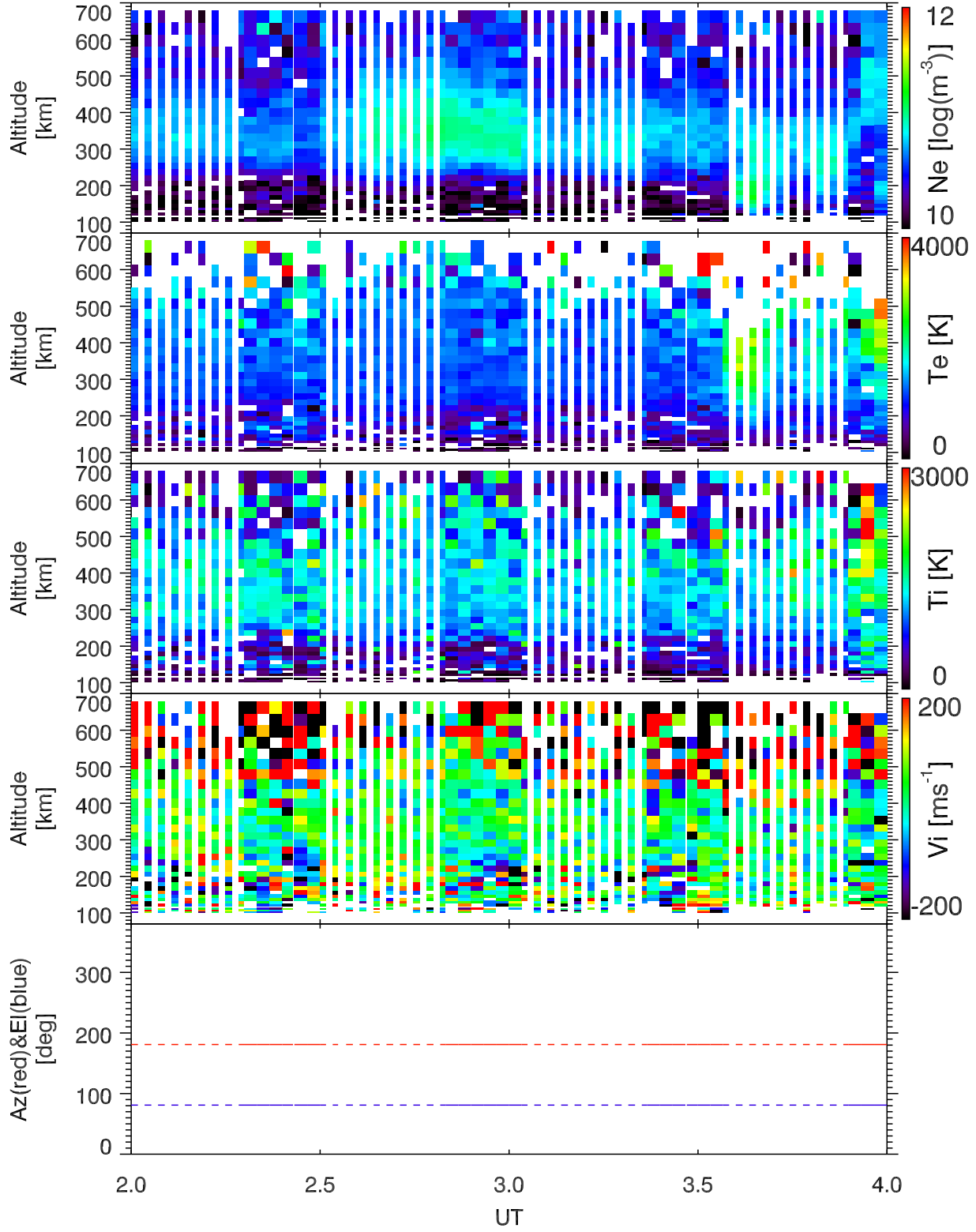
EISCAT 2001-12-13_02_04UT_tau0_120@42m.
