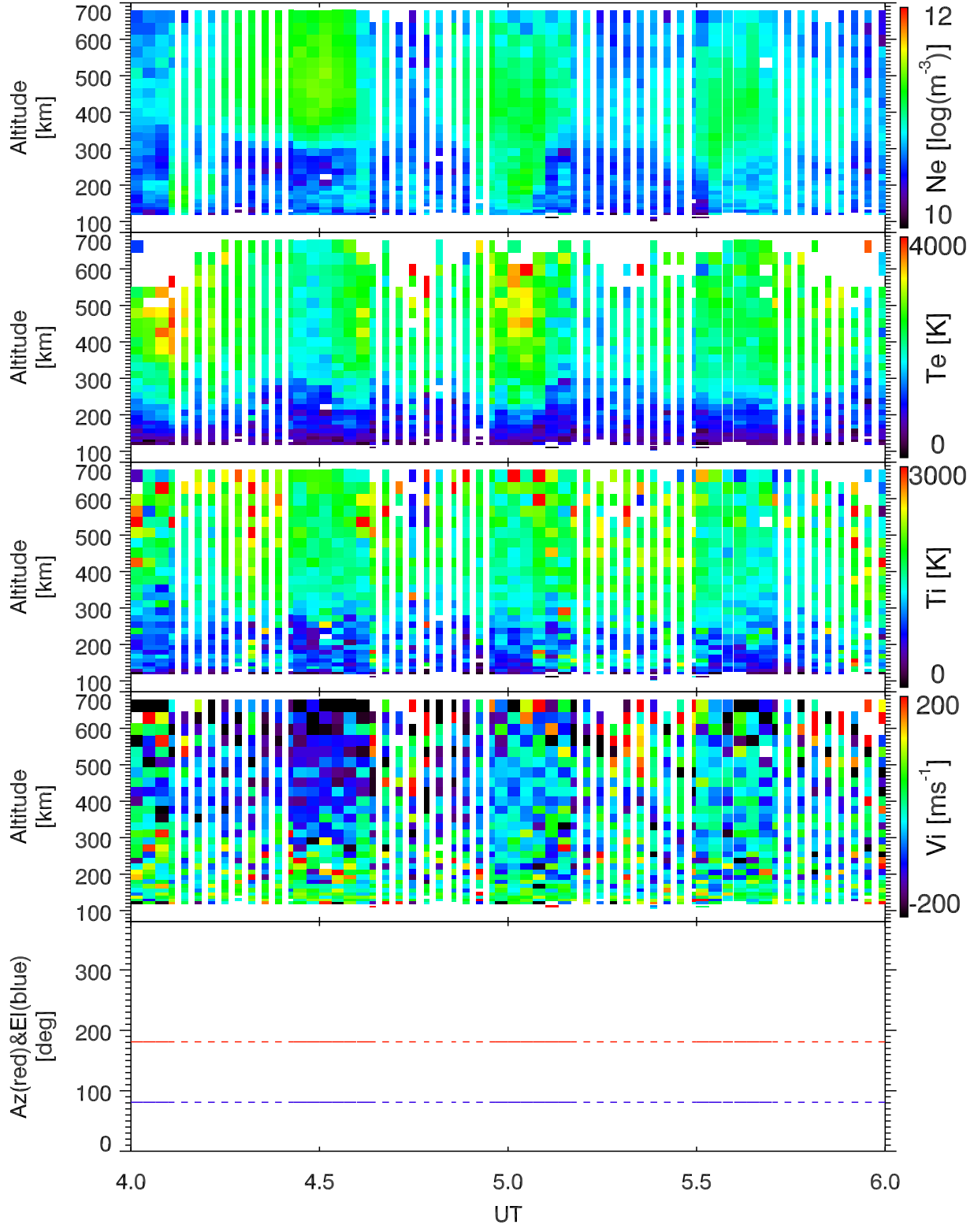
EISCAT 2001-12-13_04_06UT_tau0_120@42m.
