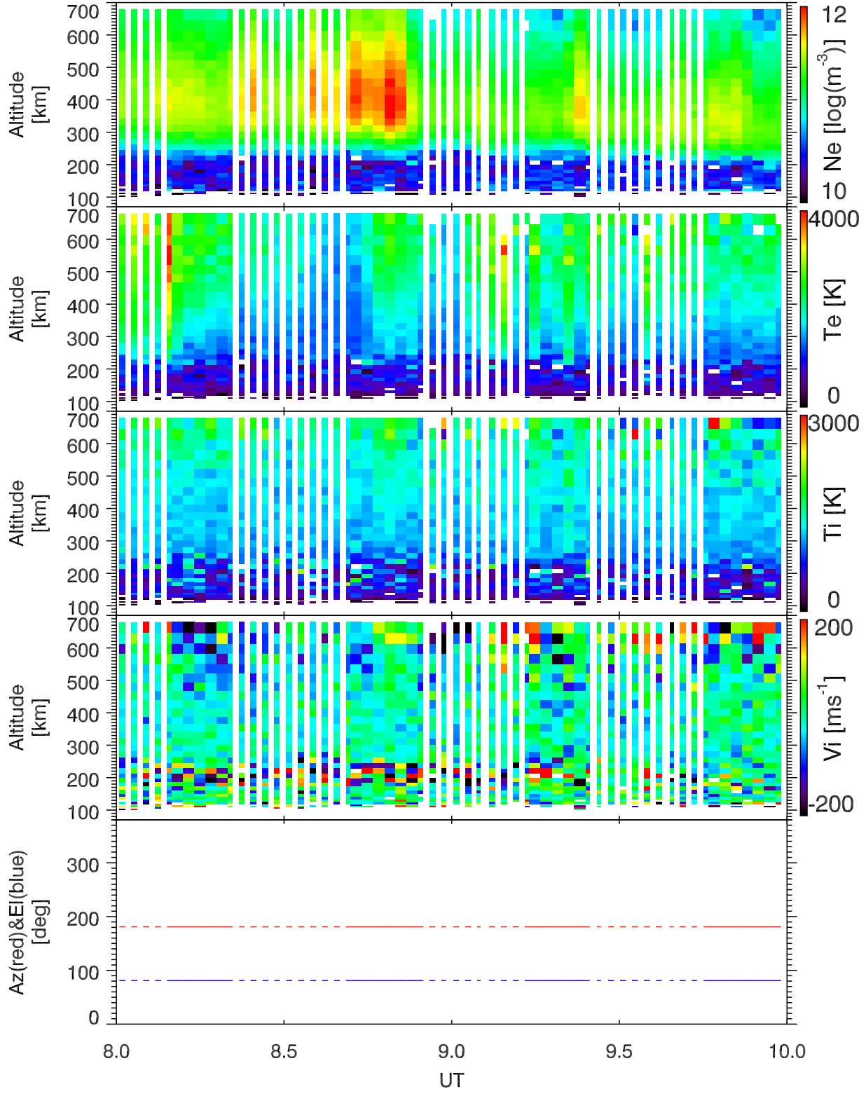
EISCAT 2001-12-13_08_10UT_tau0_120@42m.
