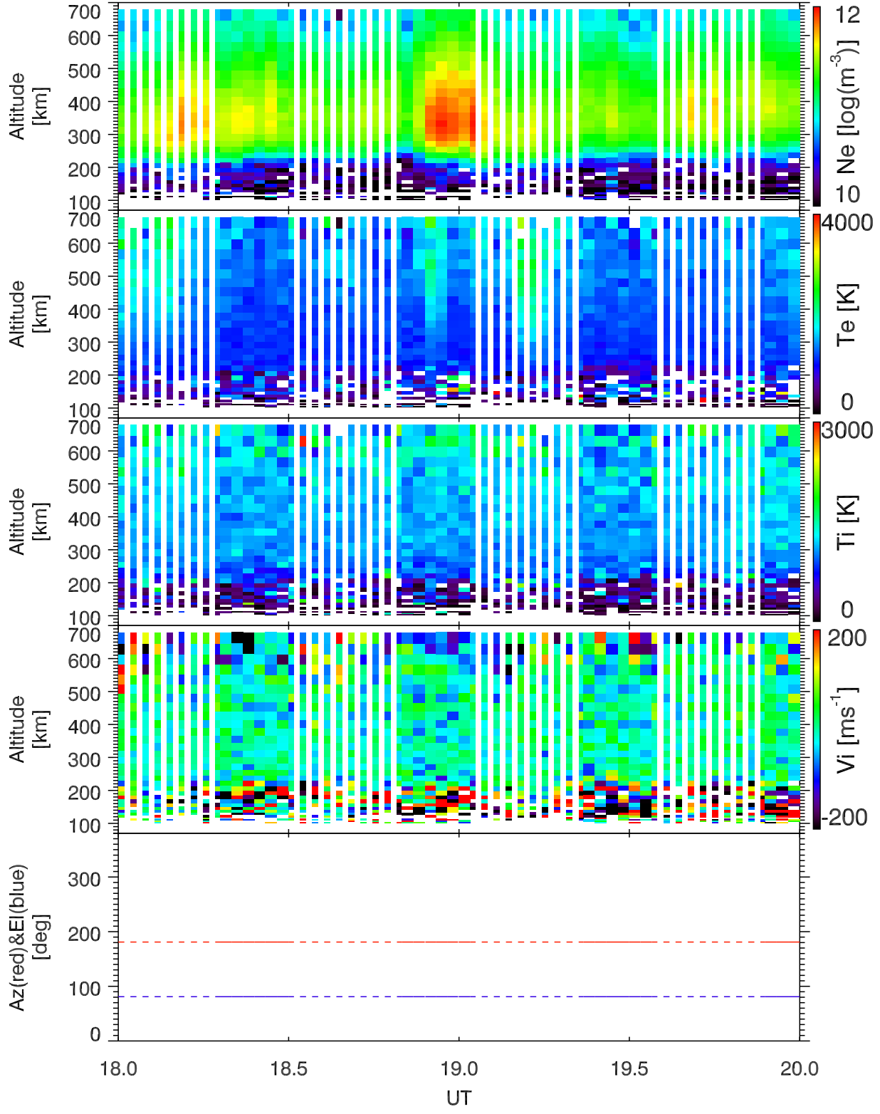
EISCAT 2001-12-13_18_20UT_tau0_120@42m.
