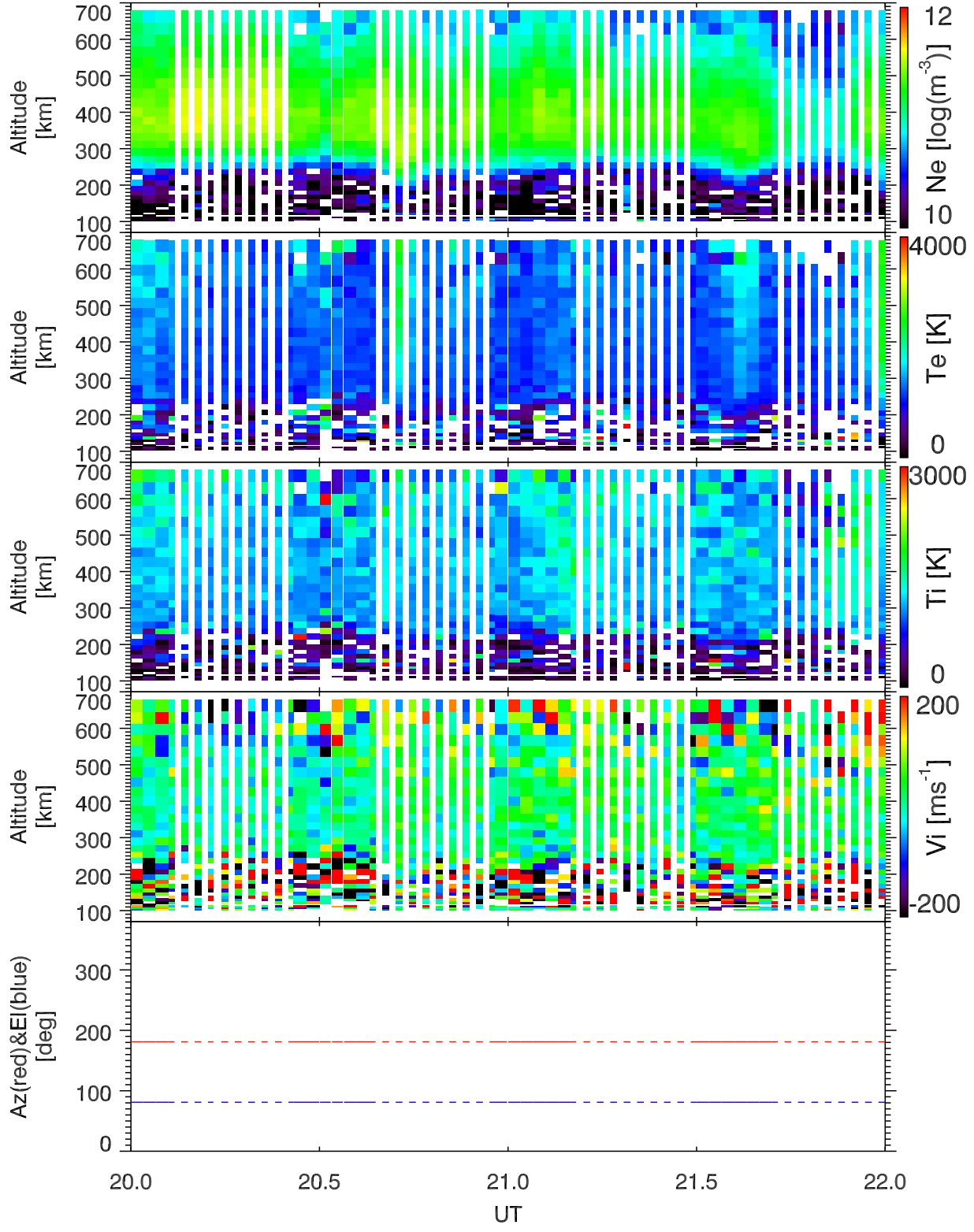
EISCAT 2001-12-13_20_22UT_tau0_120@42m.
