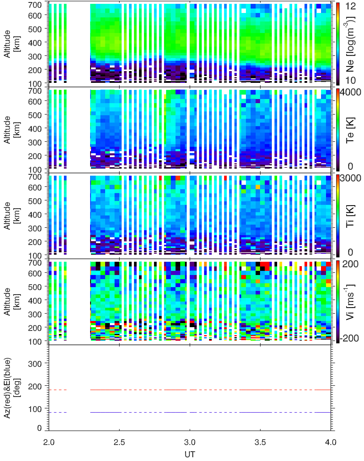
EISCAT 2001-12-14_02_04UT_tau0_120@42m.
