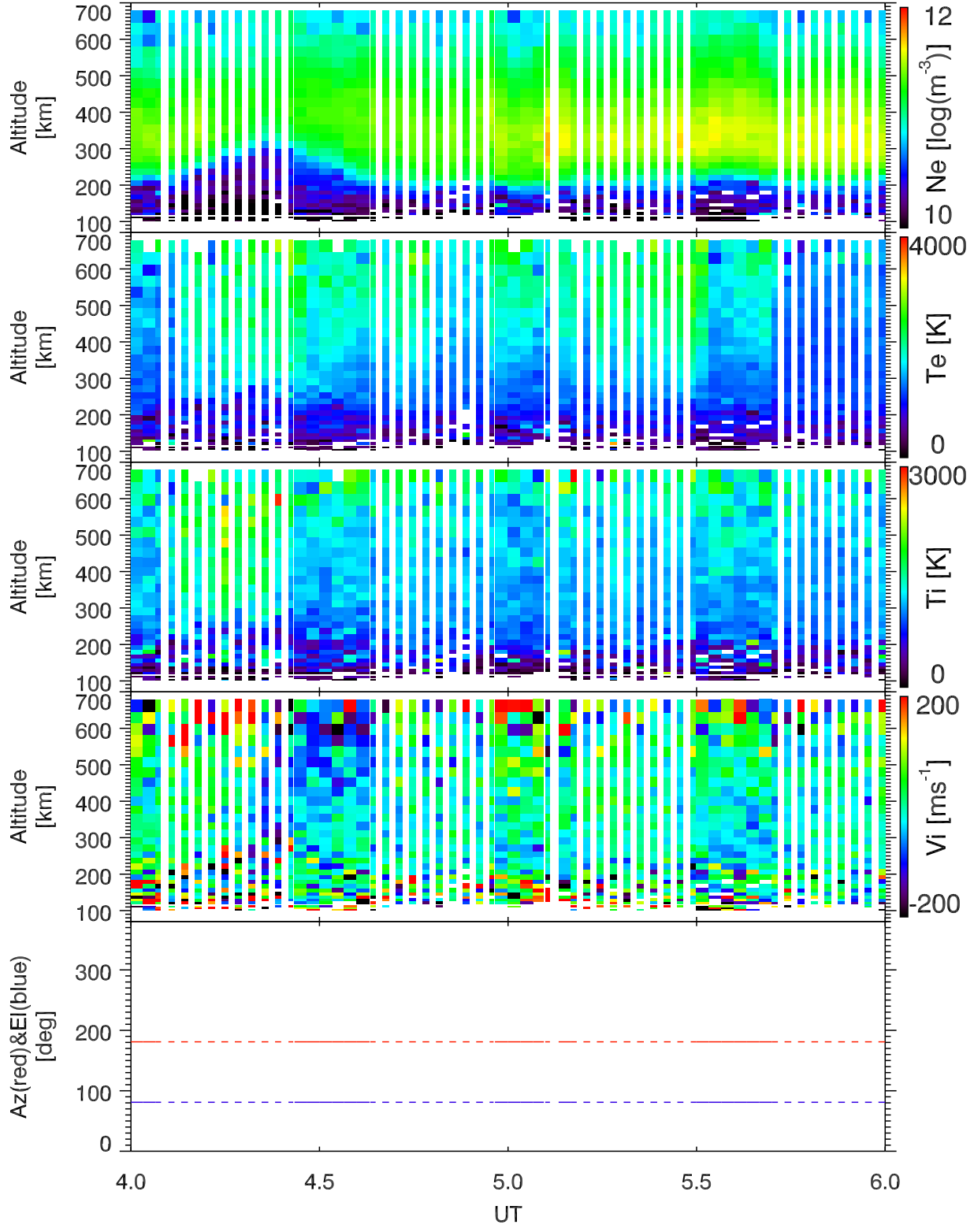
EISCAT 2001-12-14_04_06UT_tau0_120@42m.
