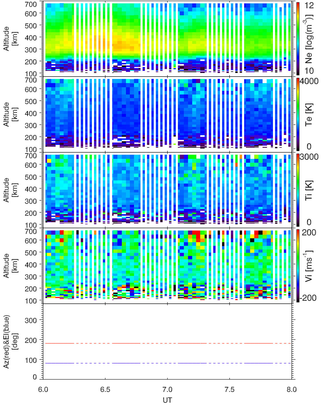
EISCAT 2001-12-14_06_08UT_tau0_120@42m.
