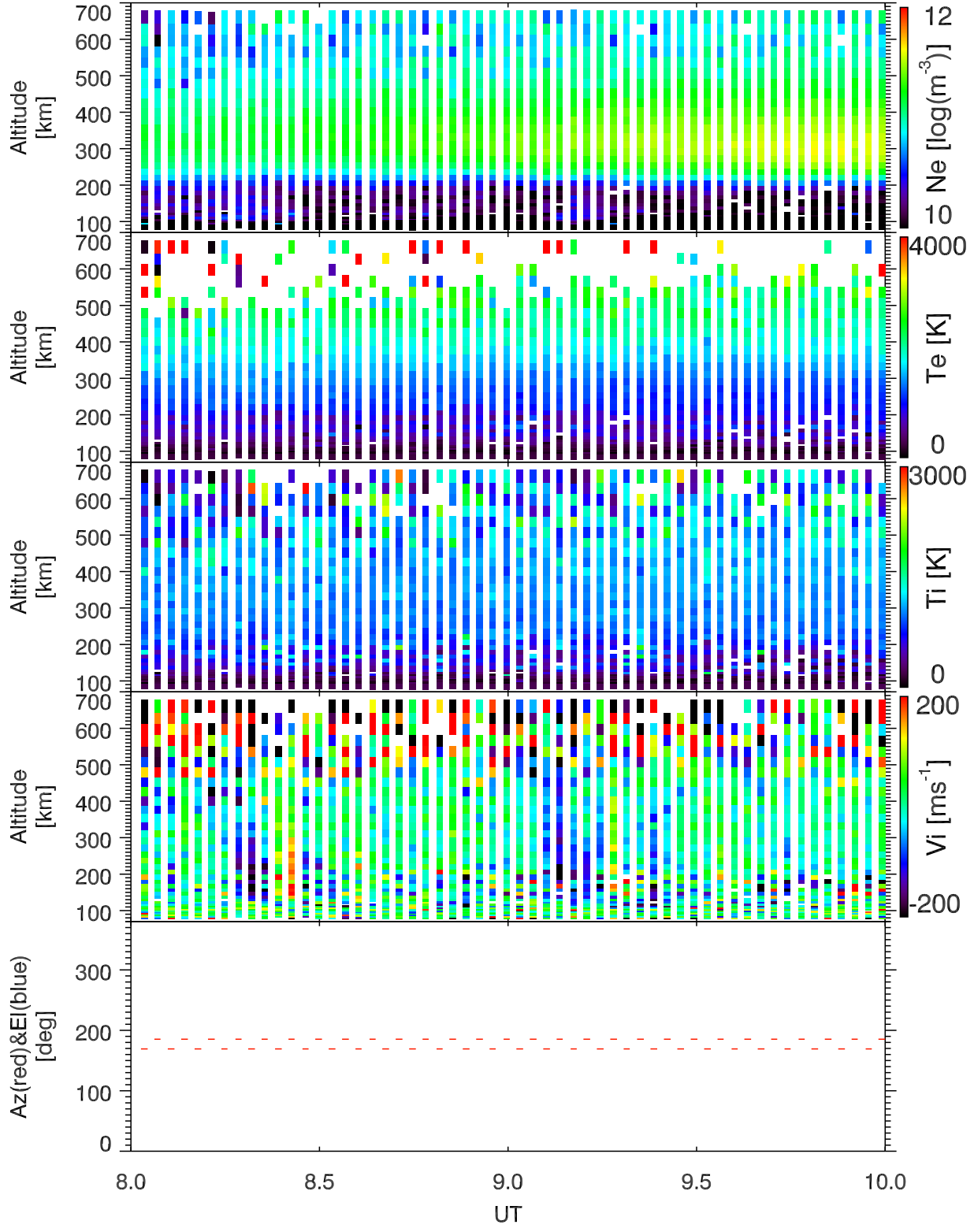
EISCAT 2001-12-14_08_10UT_tau0_ant@32m.
