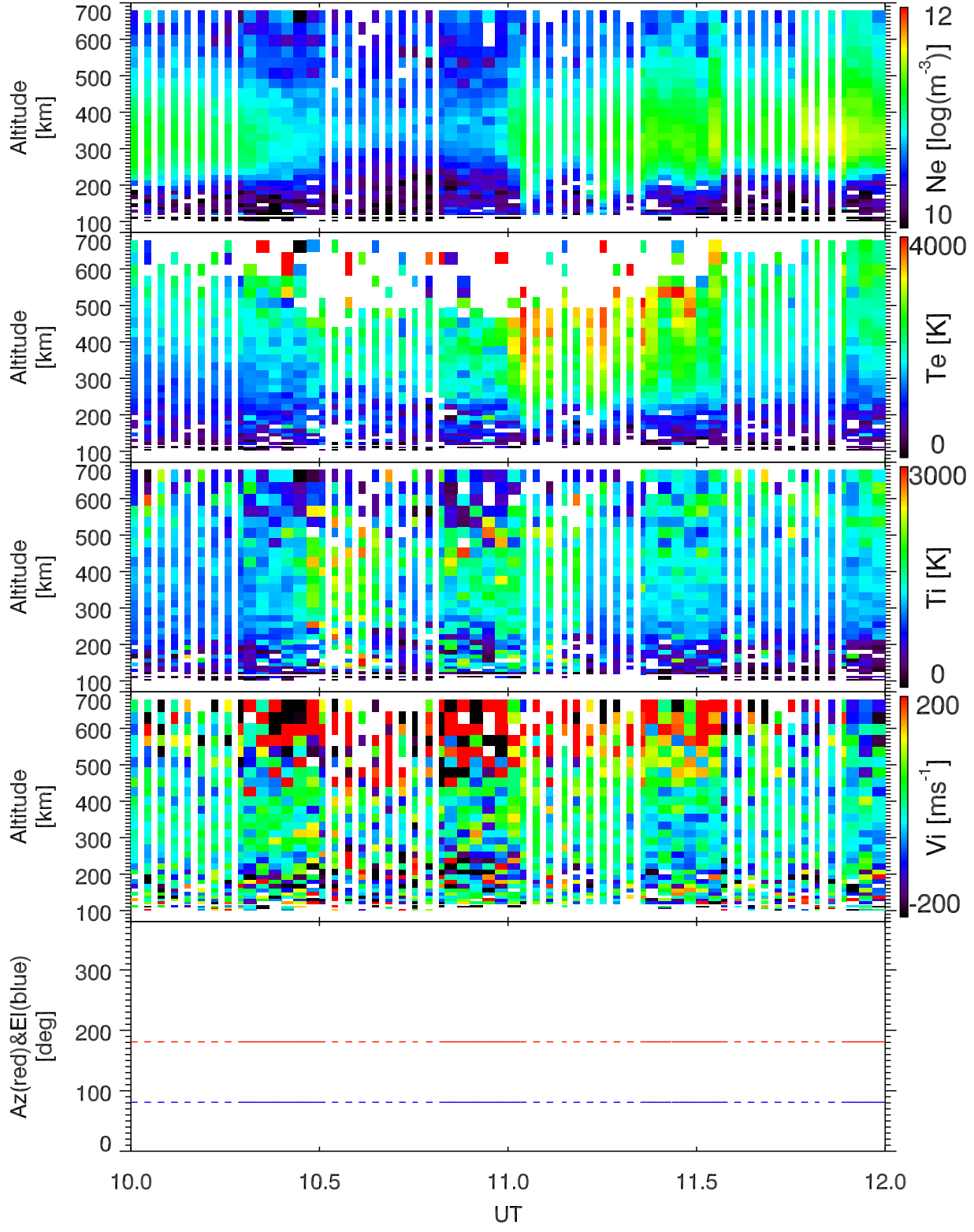
EISCAT 2001-12-14_10_12UT_tau0_120@42m.
