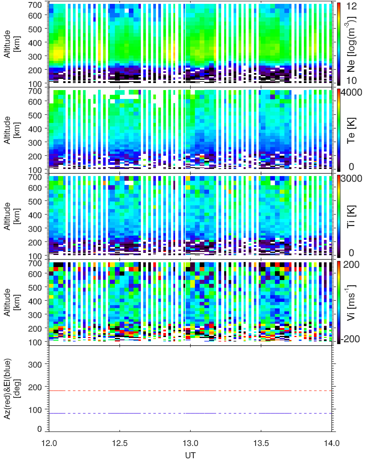
EISCAT 2001-12-14_12_14UT_tau0_120@42m.
