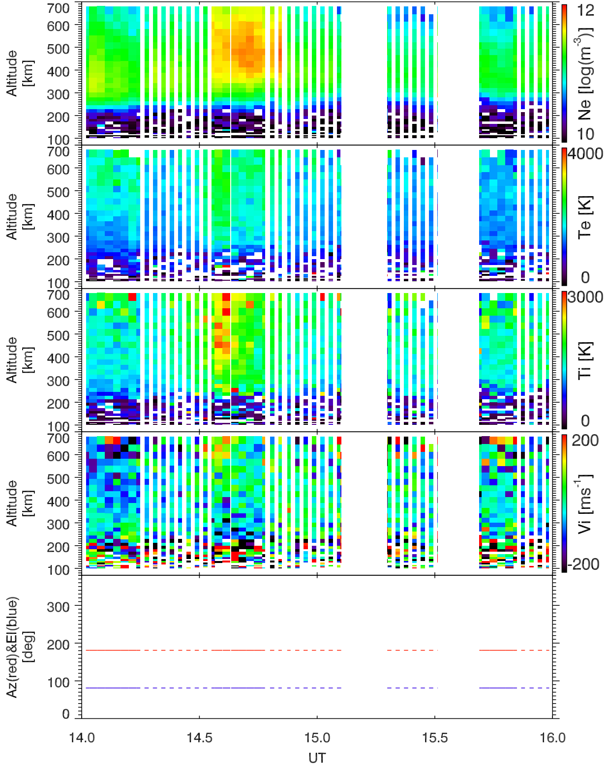
EISCAT 2001-12-14_14_16UT_tau0_120@42m.
