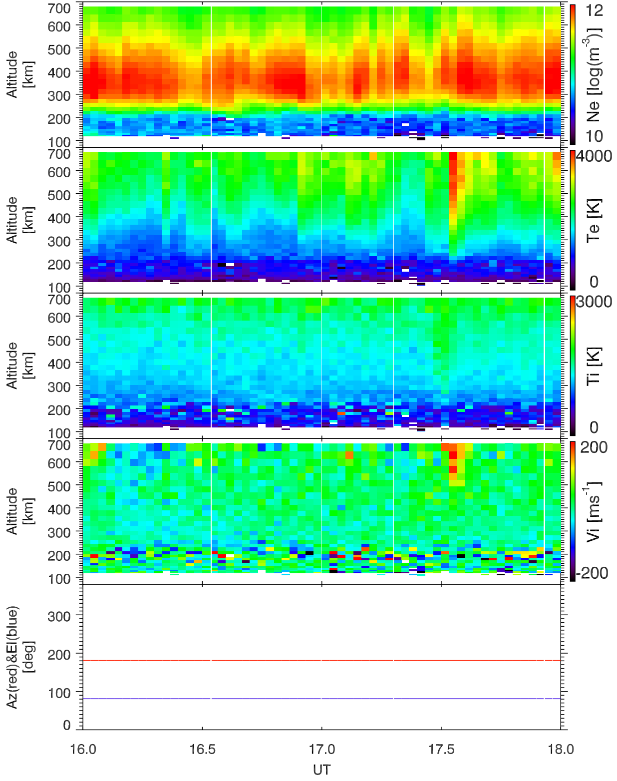
EISCAT 2001-12-15_16_18UT_tau0_120@42m.
