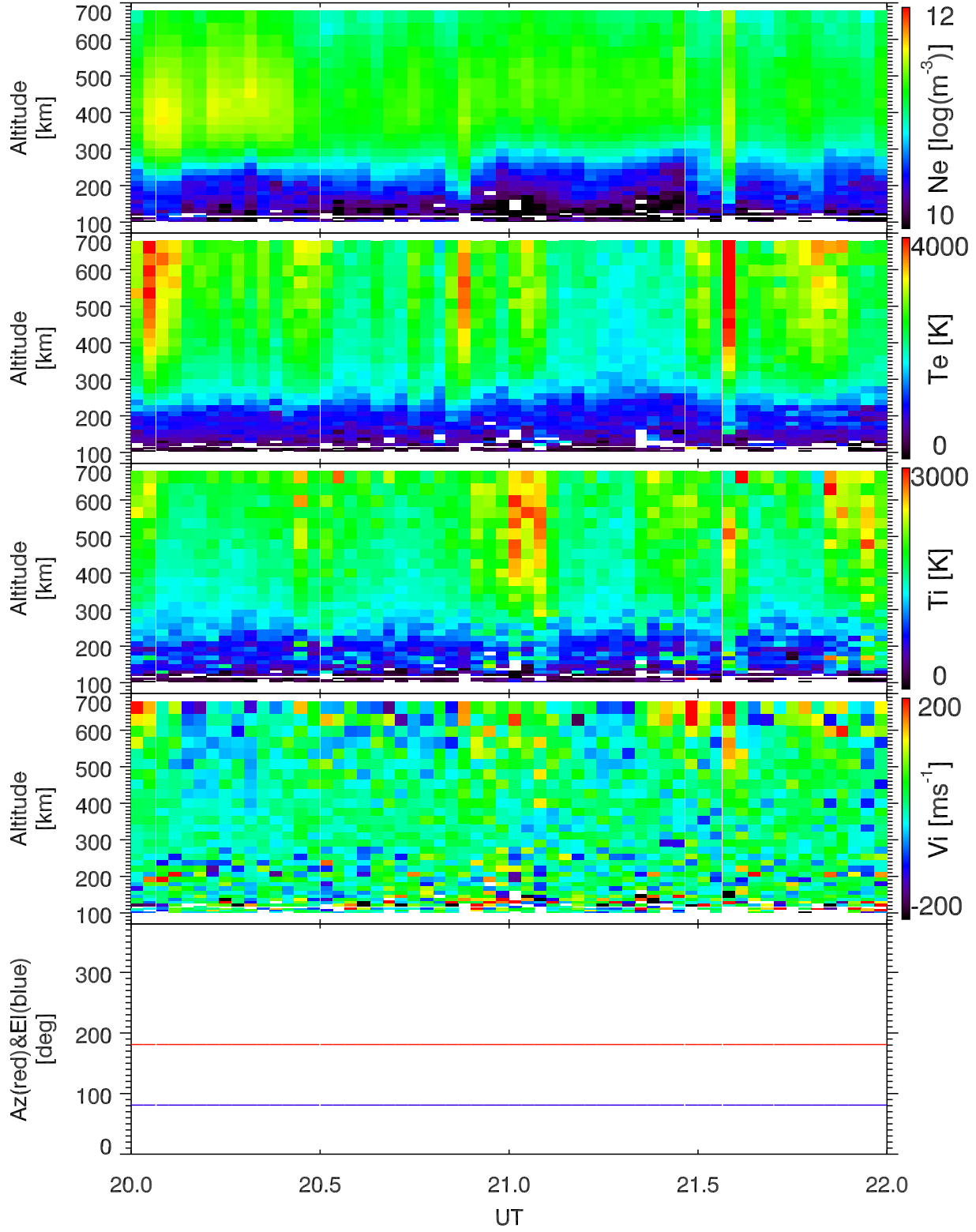
EISCAT 2001-12-15_20_22UT_tau0_120@42m.
