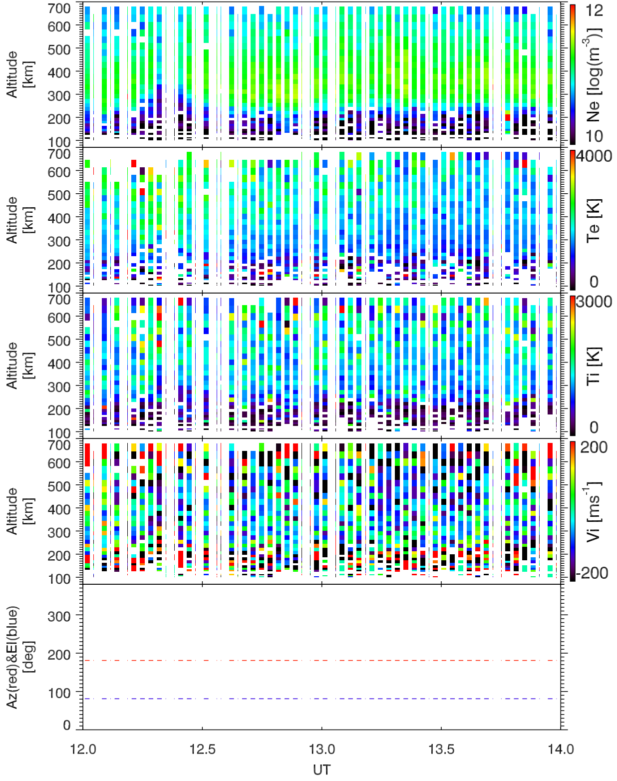
EISCAT 2001-12-18_12_14UT_tau0_120@42m.
