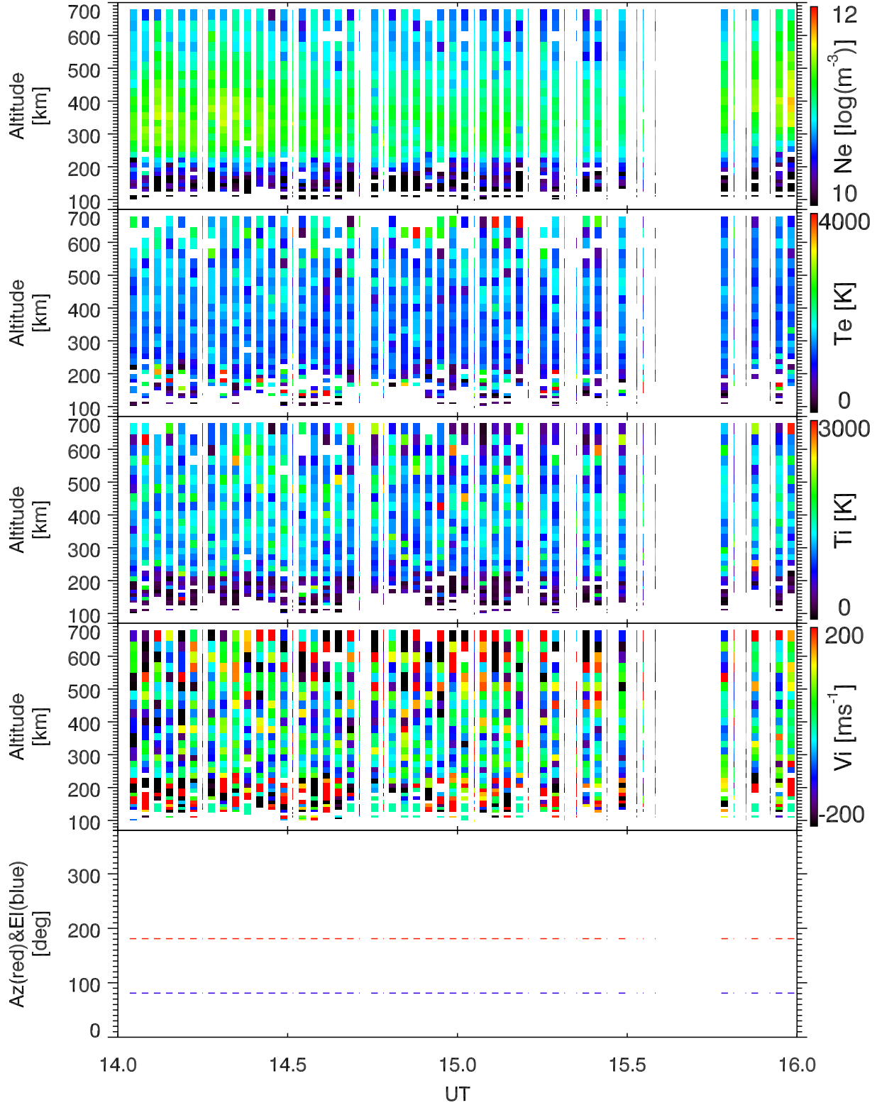
EISCAT 2001-12-18_14_16UT_tau0_120@42m.
