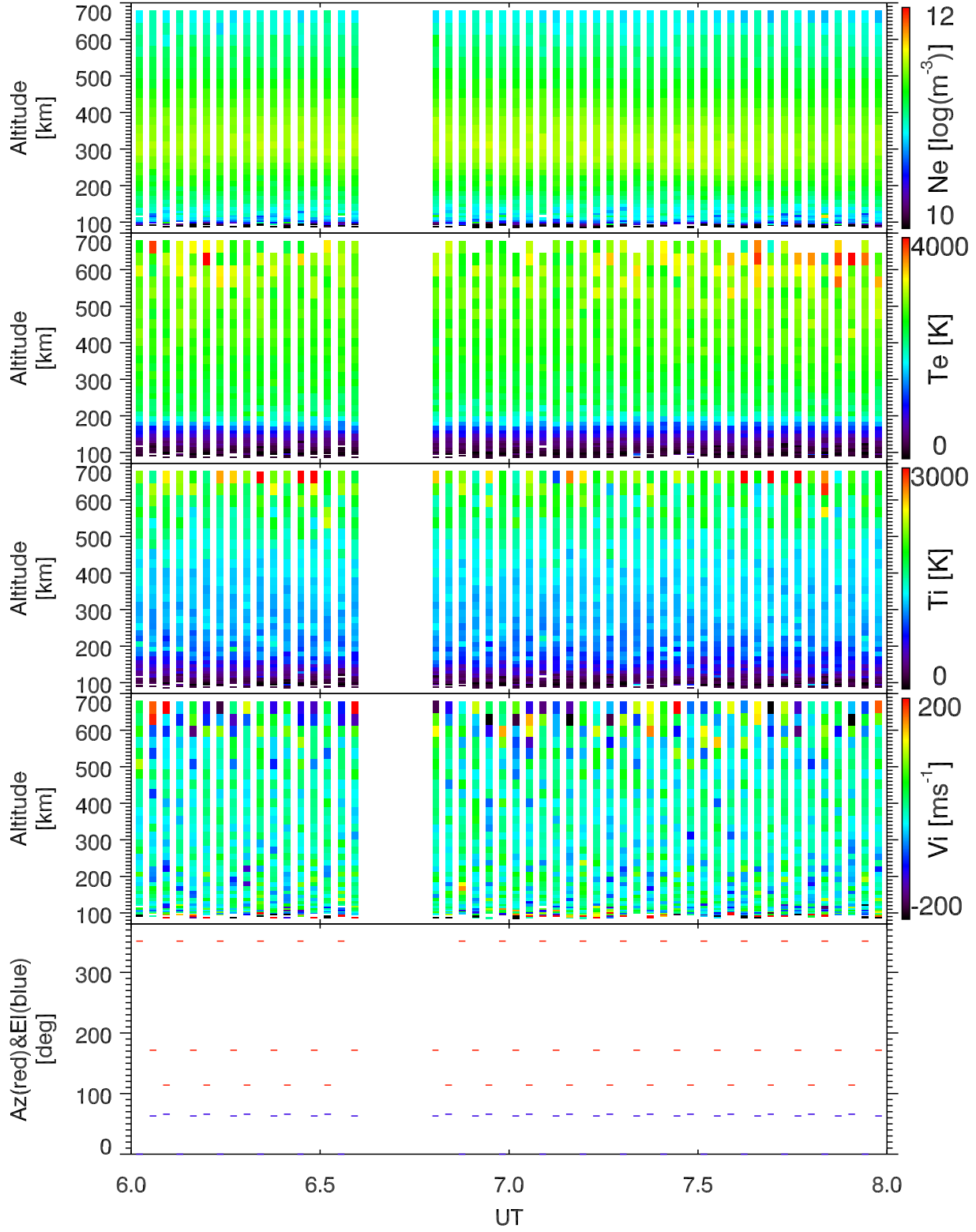
EISCAT 2002-07-15_06_08UT_tau0_ant@32m.
