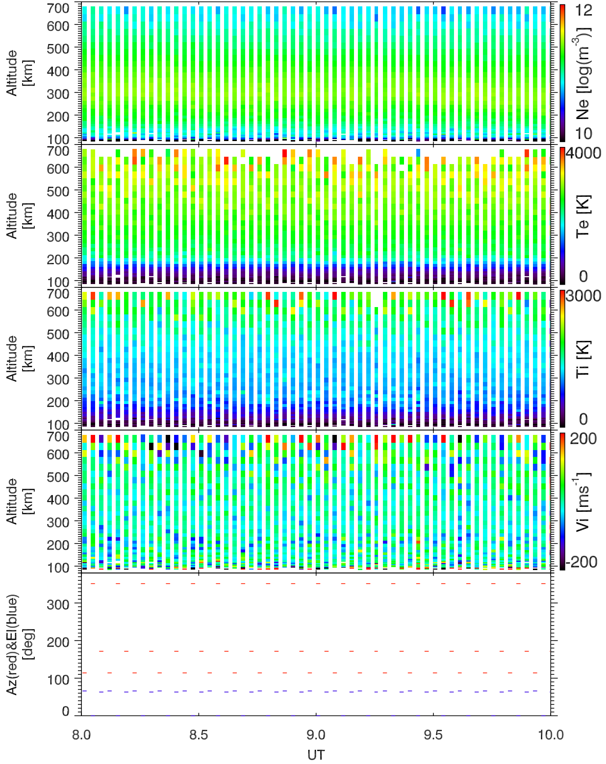
EISCAT 2002-07-15_08_10UT_tau0_ant@32m.
