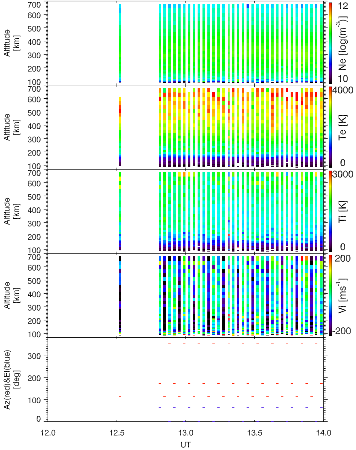
EISCAT 2002-07-24_12_14UT_tau0_ant@32m.
