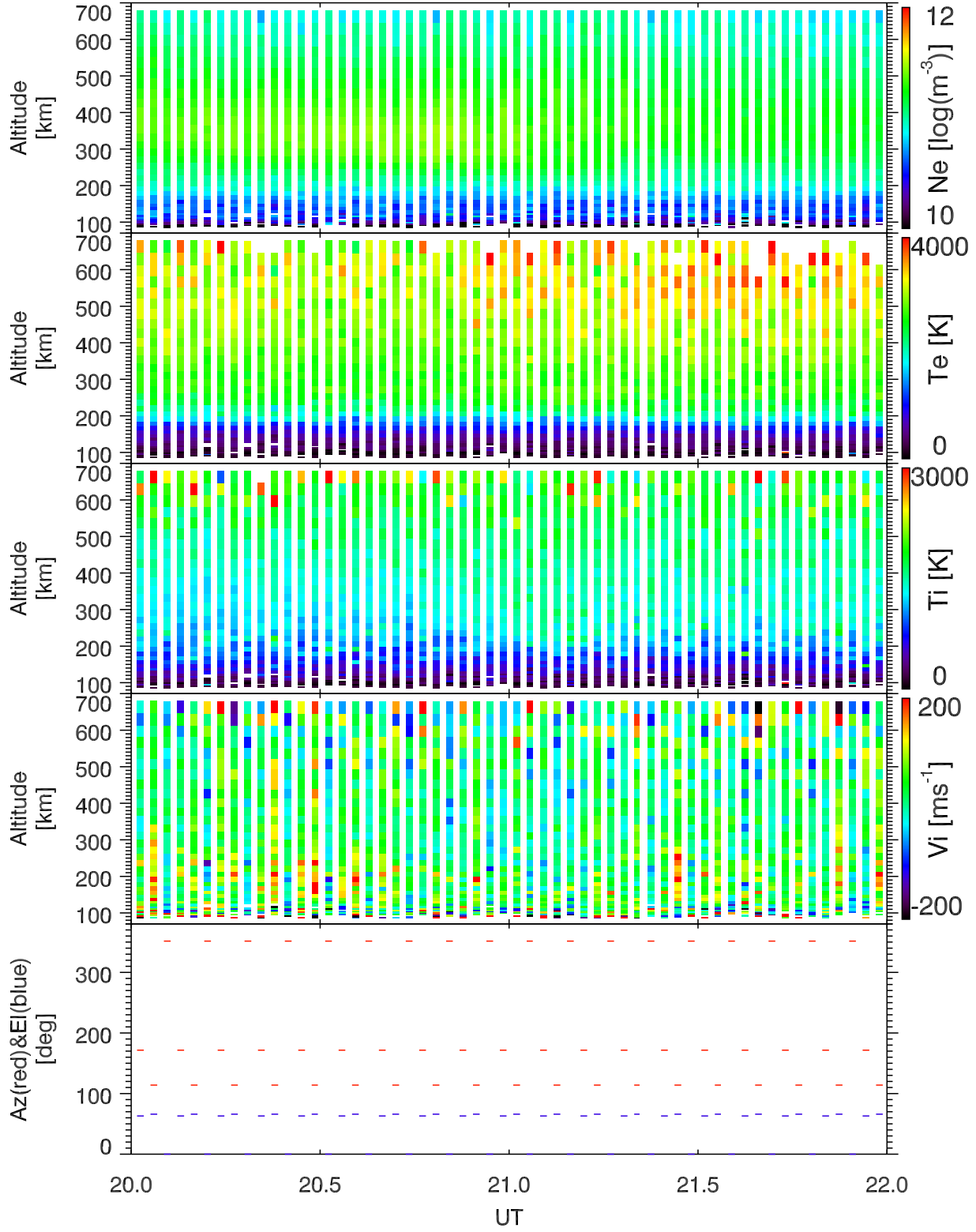
EISCAT 2002-07-29_20_22UT_tau0_ant@32m.
