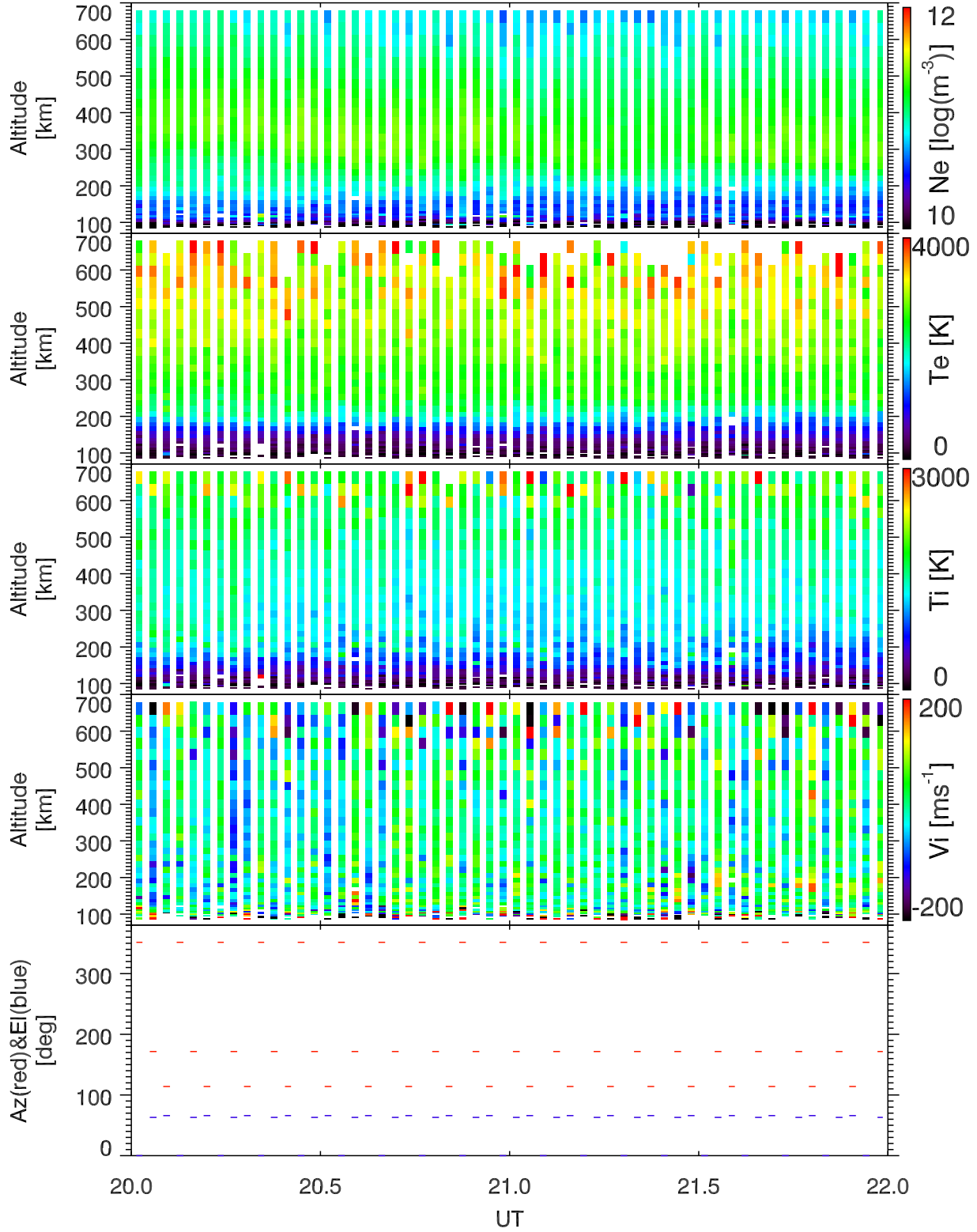
EISCAT 2002-07-31_20_22UT_tau0_ant@32m.
