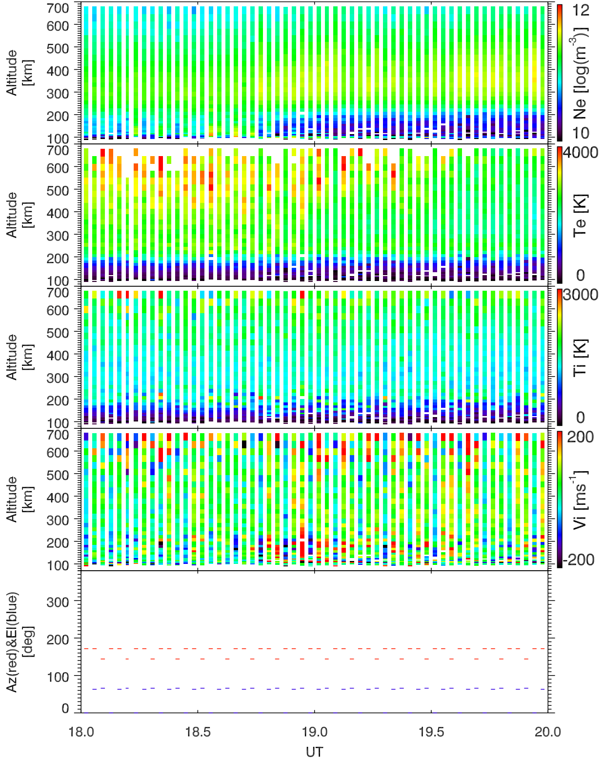
EISCAT 2002-08-30_18_20UT_tau0_ant@32m.
