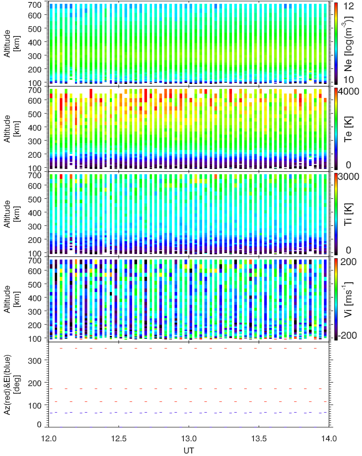
EISCAT 2002-09-01_12_14UT_tau0_ant@32m.
