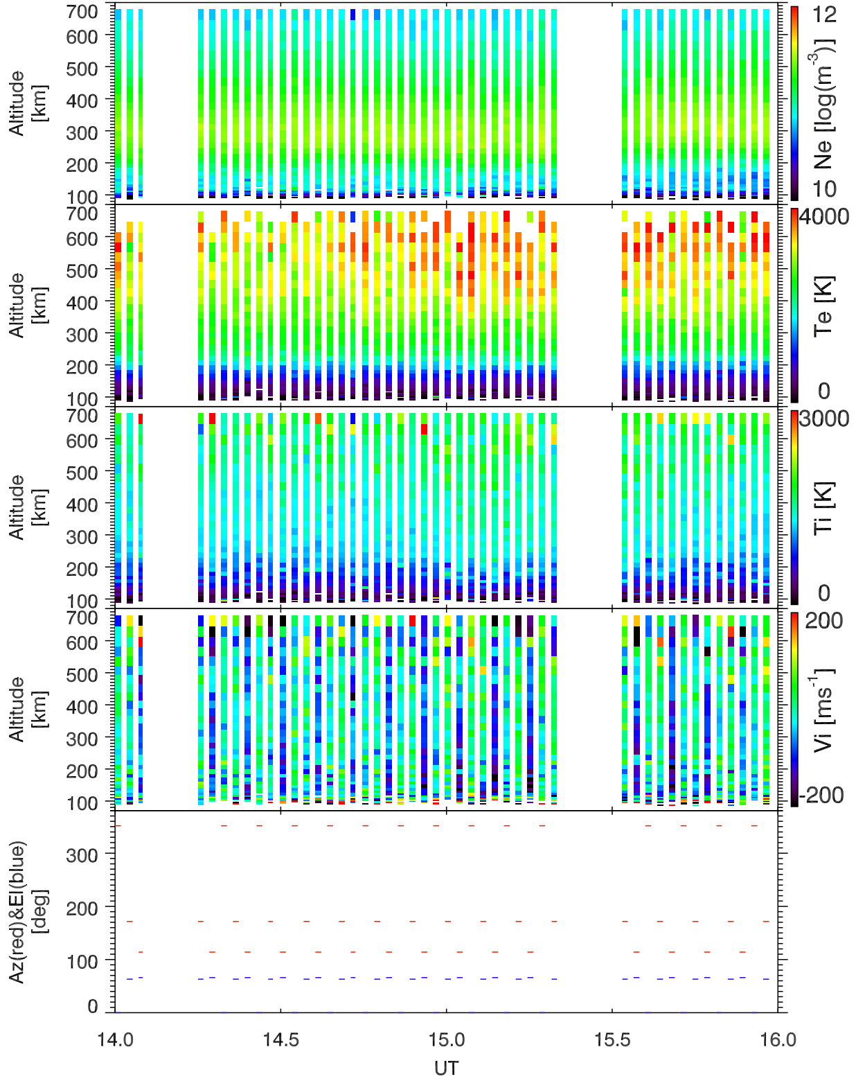
EISCAT 2002-09-01_14_16UT_tau0_ant@32m.
