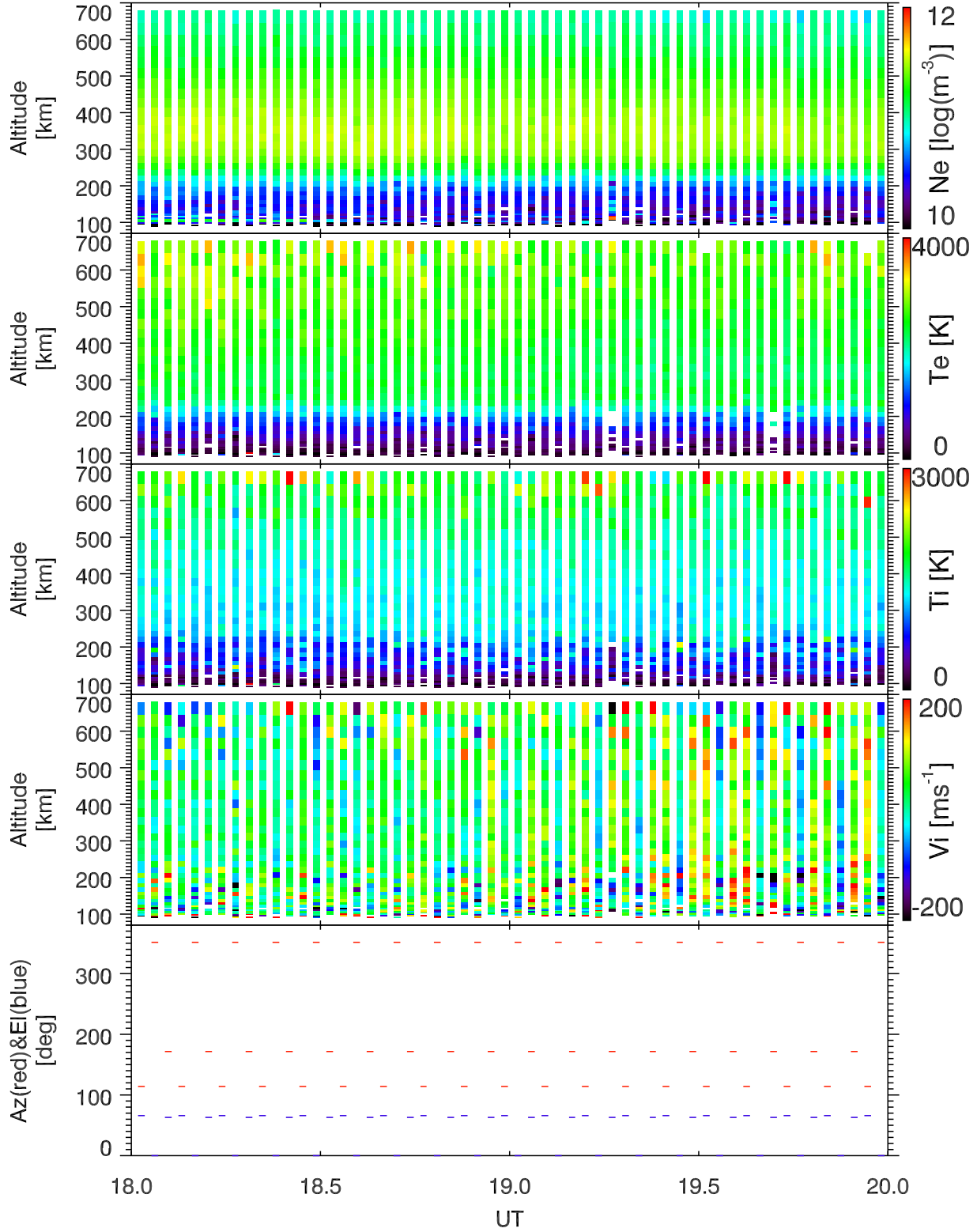
EISCAT 2002-09-01_18_20UT_tau0_ant@32m.
