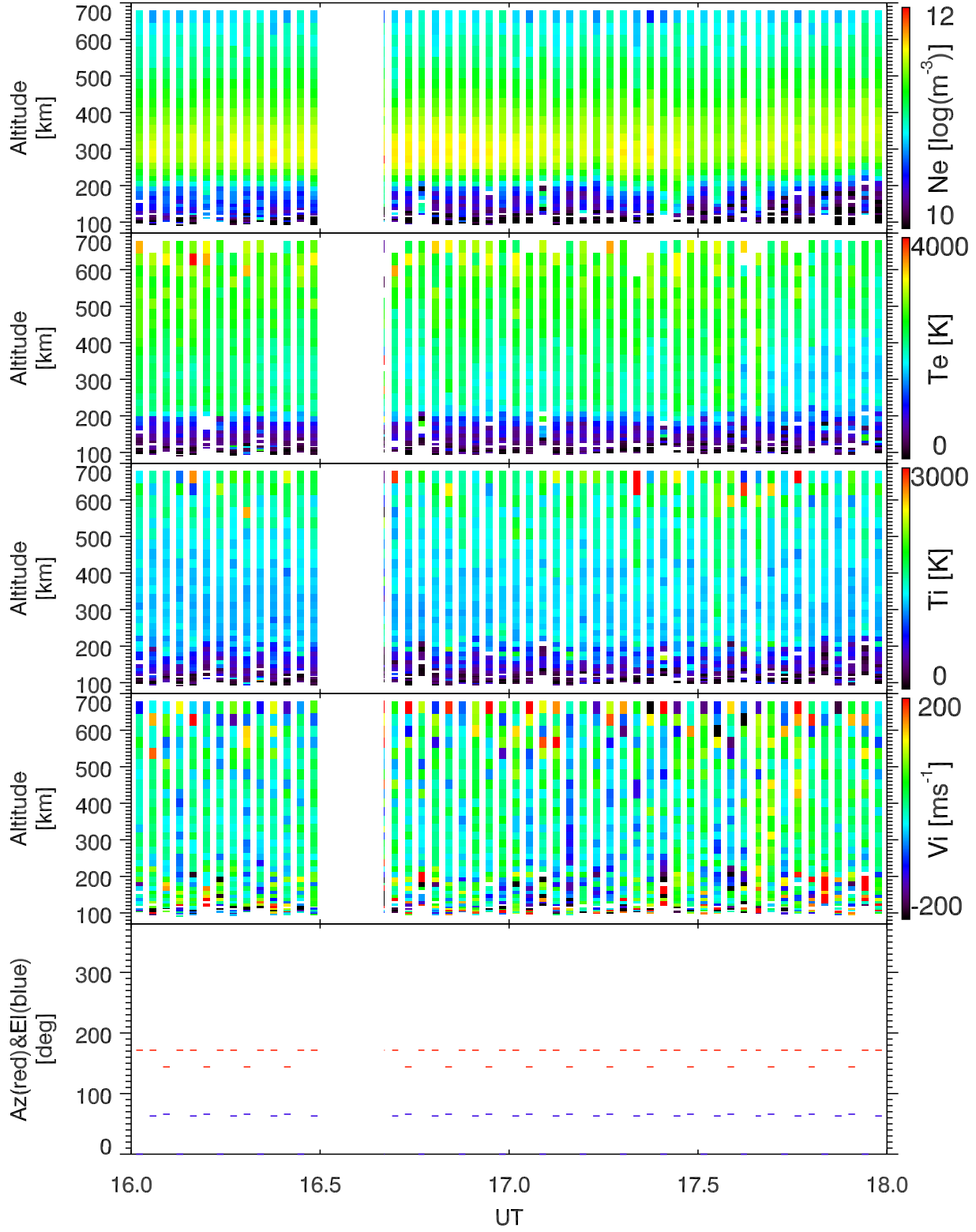
EISCAT 2002-09-25_16_18UT_tau0_ant@32m.
