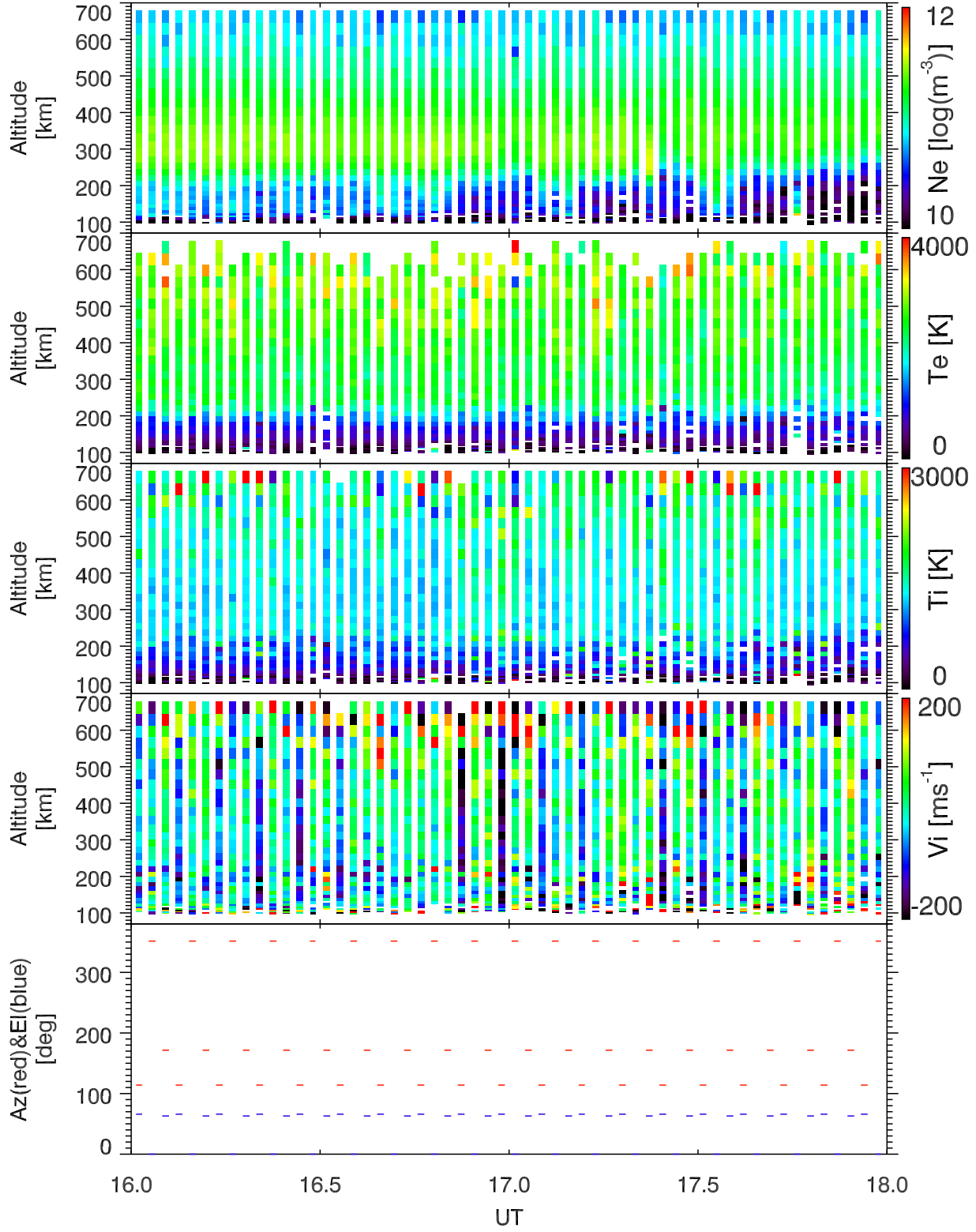
EISCAT 2002-09-27_16_18UT_tau0_ant@32m.
