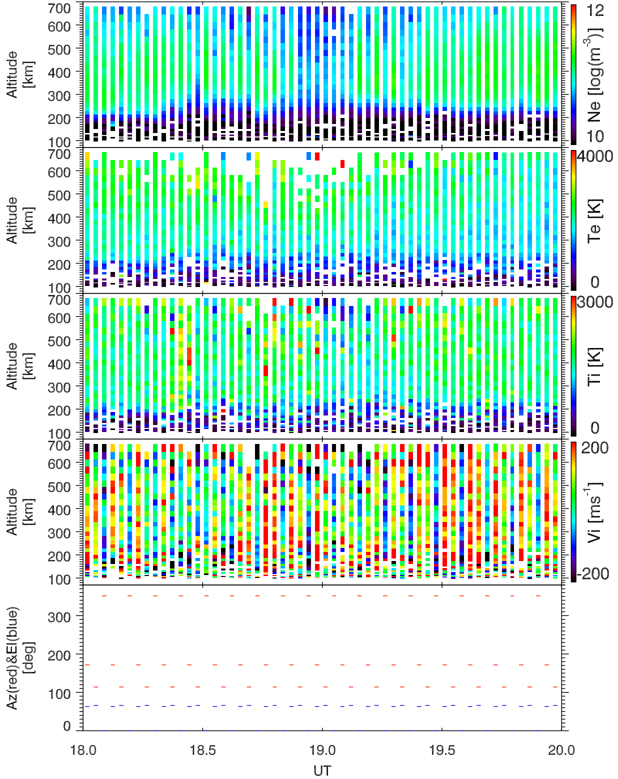
EISCAT 2002-10-04_18_20UT_tau0_ant@32m.
