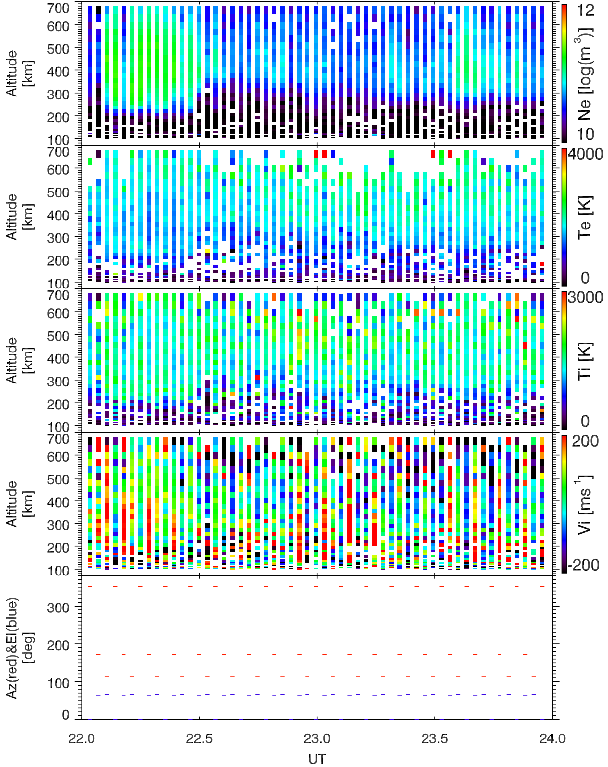
EISCAT 2002-10-04_22_24UT_tau0_ant@32m.
