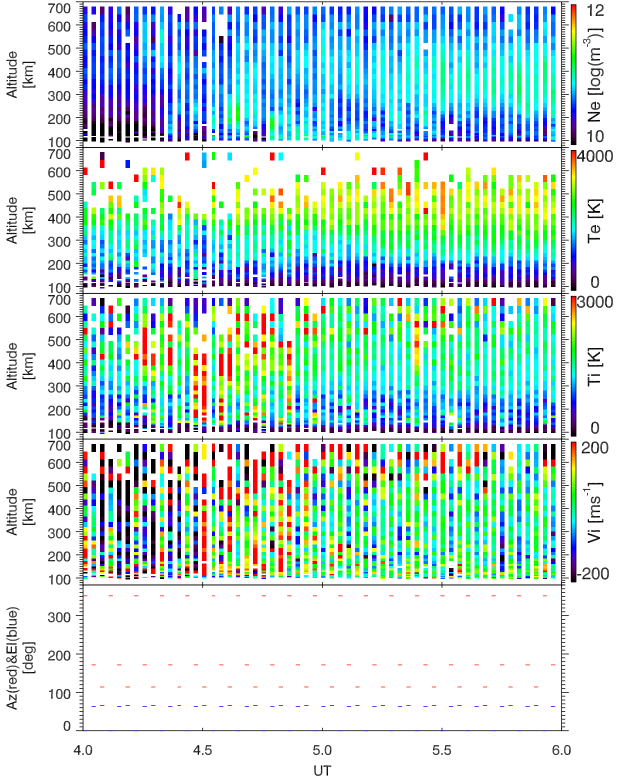
EISCAT 2002-10-05_04_06UT_tau0_ant@32m.
