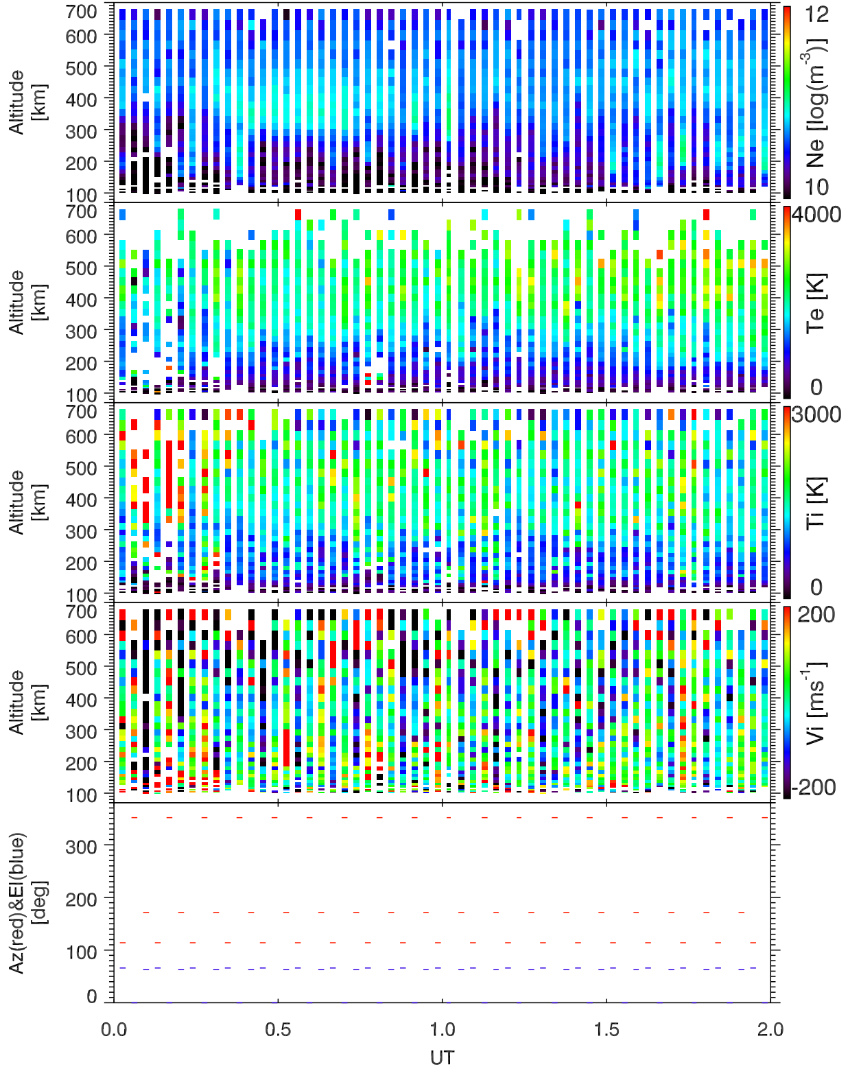
EISCAT 2002-10-06_00_02UT_tau0_ant@32m.
