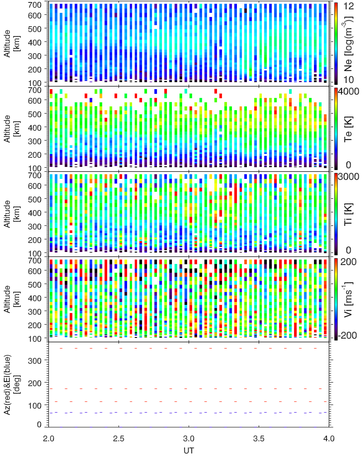
EISCAT 2002-10-06_02_04UT_tau0_ant@32m.
