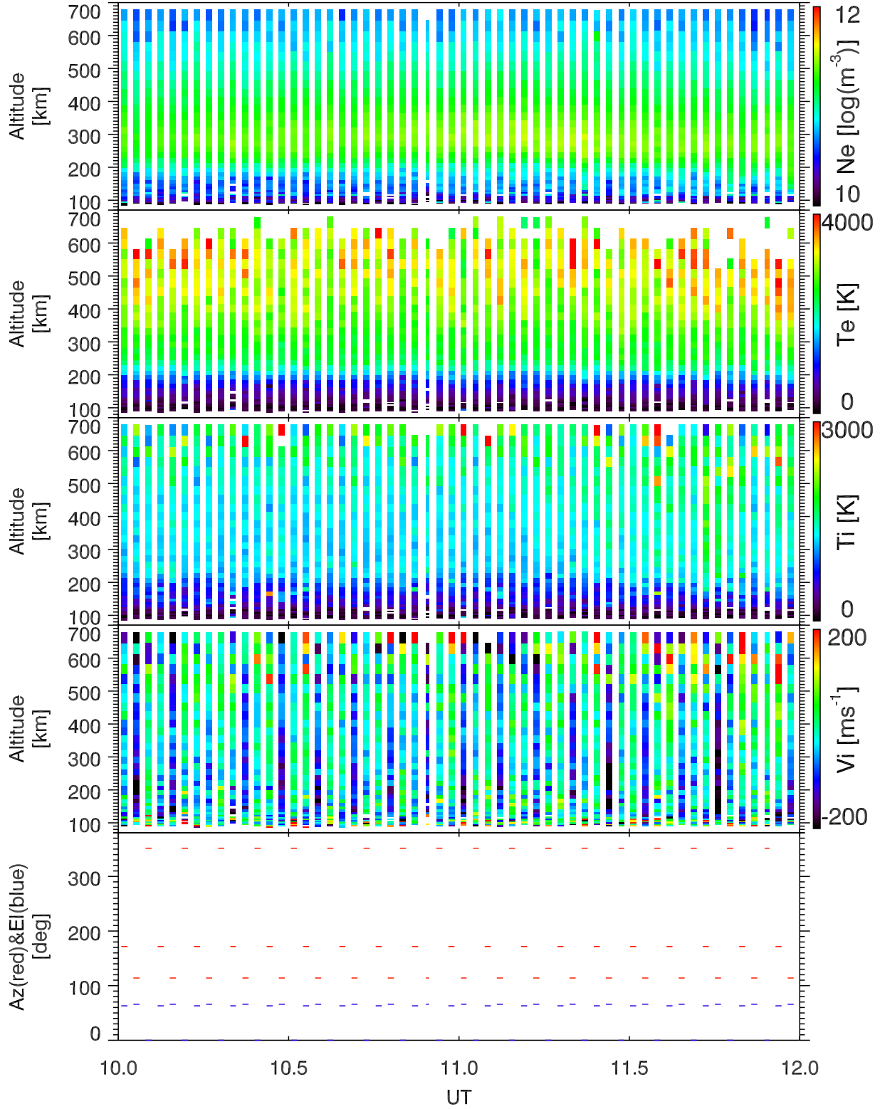
EISCAT 2002-10-06_10_12UT_tau0_ant@32m.
