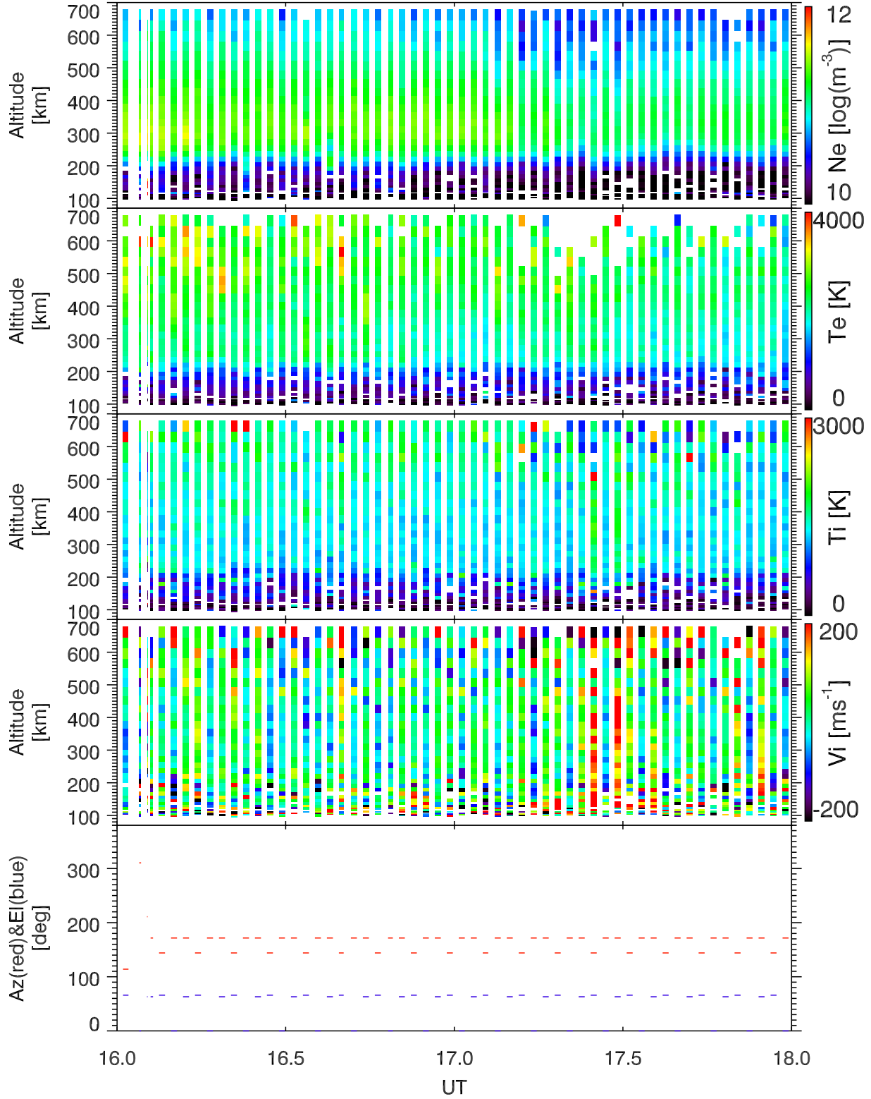
EISCAT 2002-10-06_16_18UT_tau0_ant@32m.
