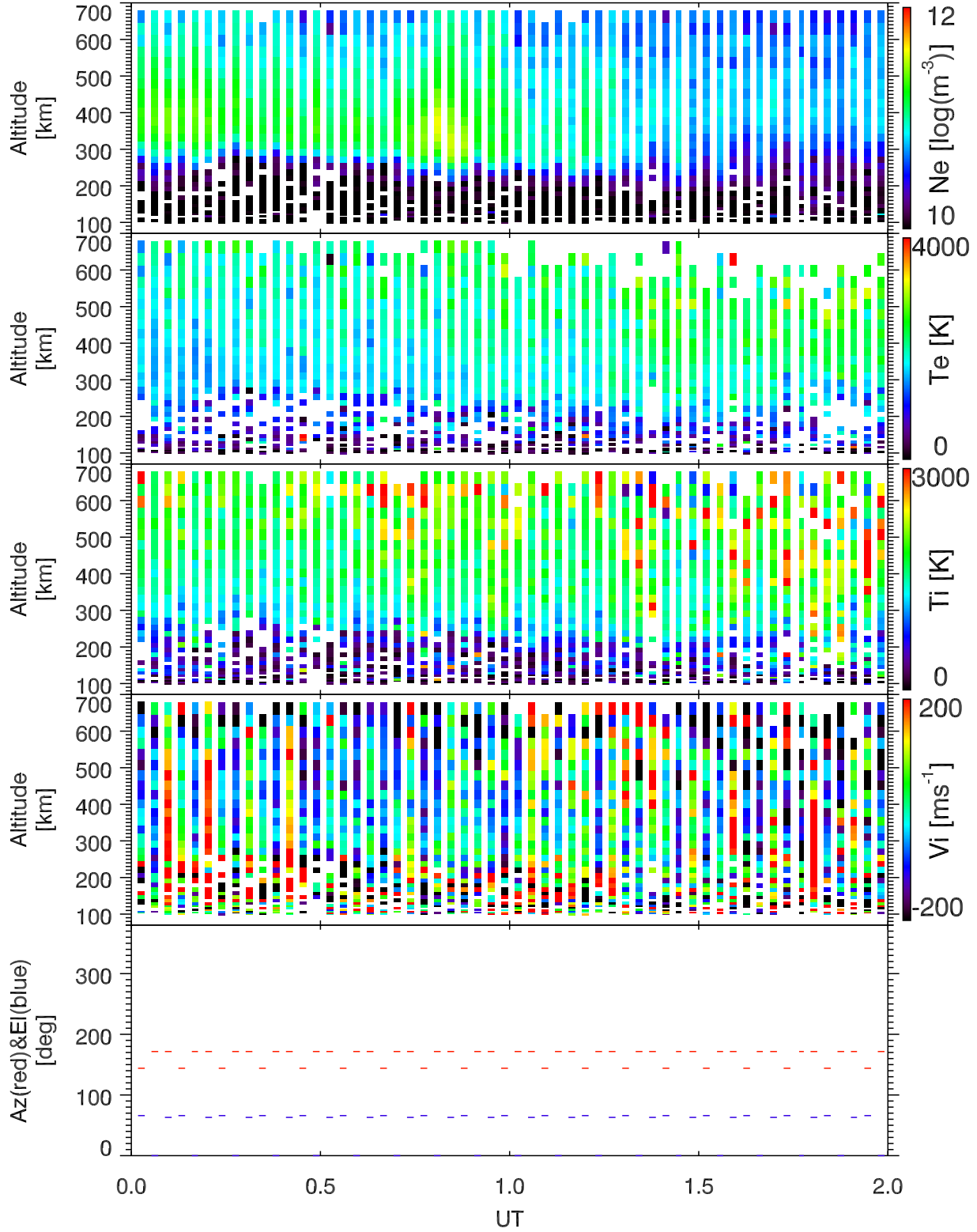
EISCAT 2002-10-07_00_02UT_tau0_ant@32m.
