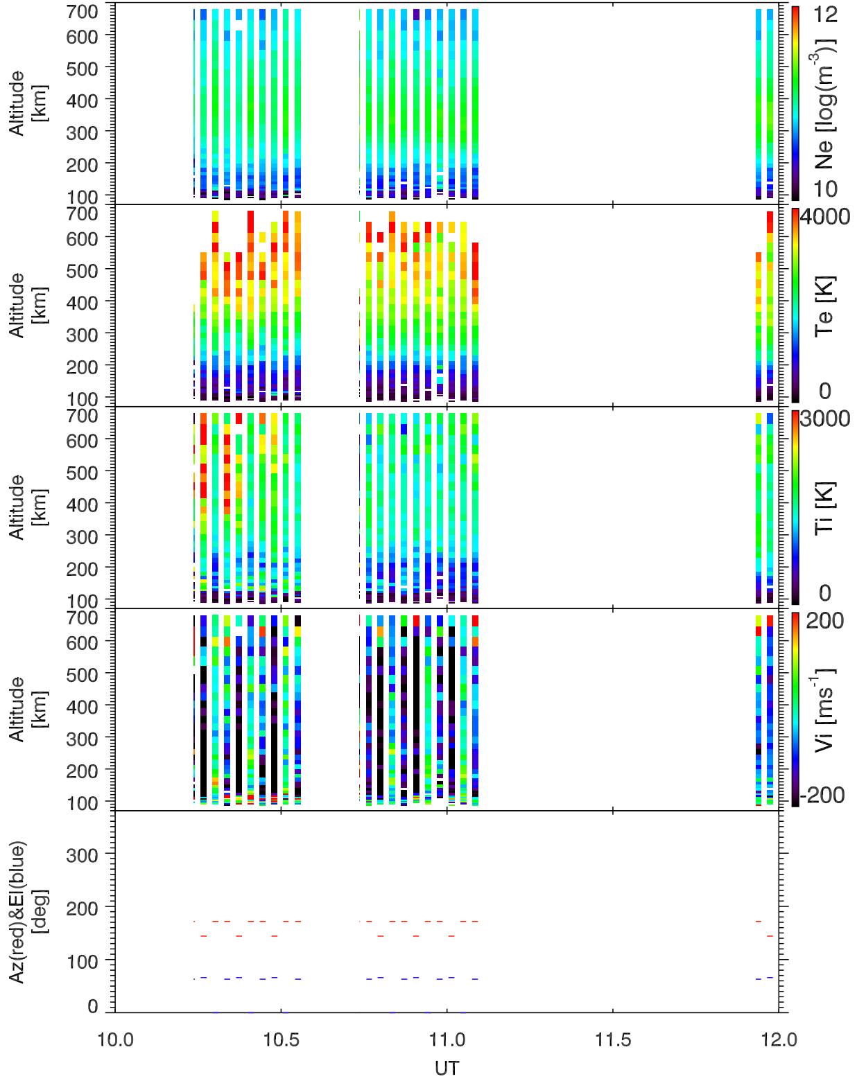
EISCAT 2002-10-07_10_12UT_tau0_ant@32m.
