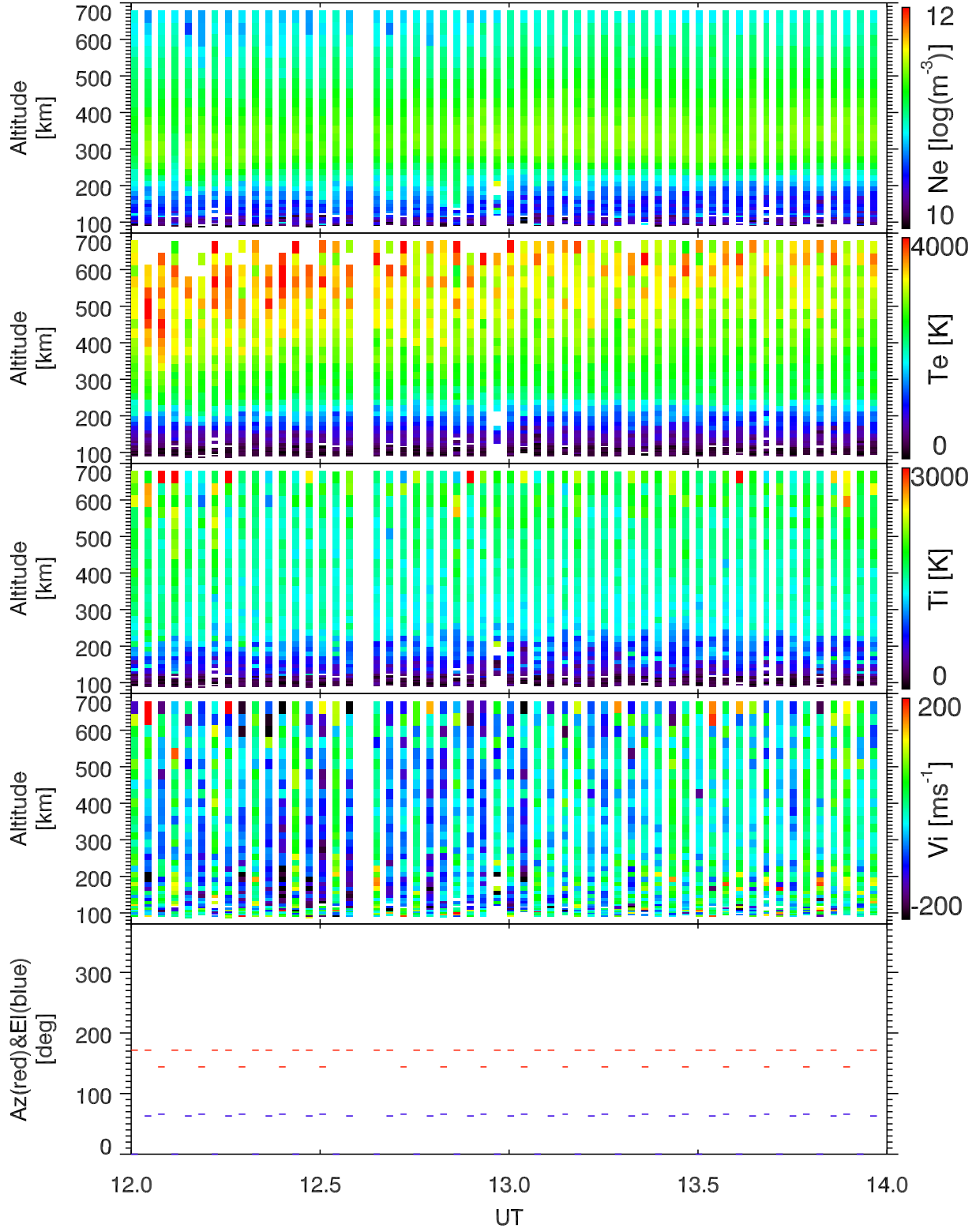
EISCAT 2002-10-07_12_14UT_tau0_ant@32m.
