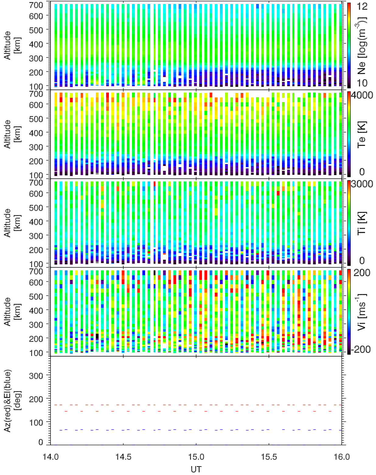
EISCAT 2002-10-07_14_16UT_tau0_ant@32m.
