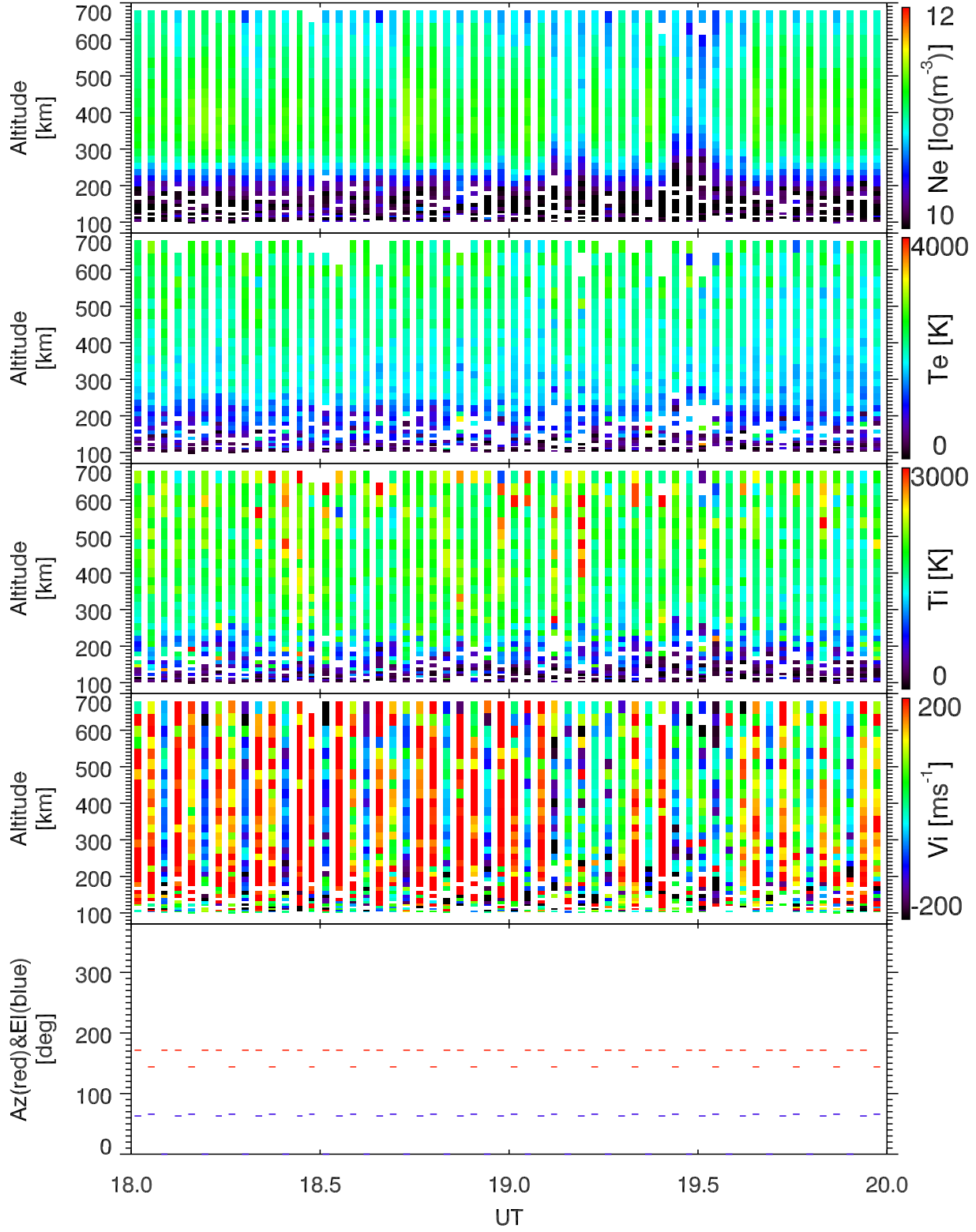
EISCAT 2002-10-07_18_20UT_tau0_ant@32m.
