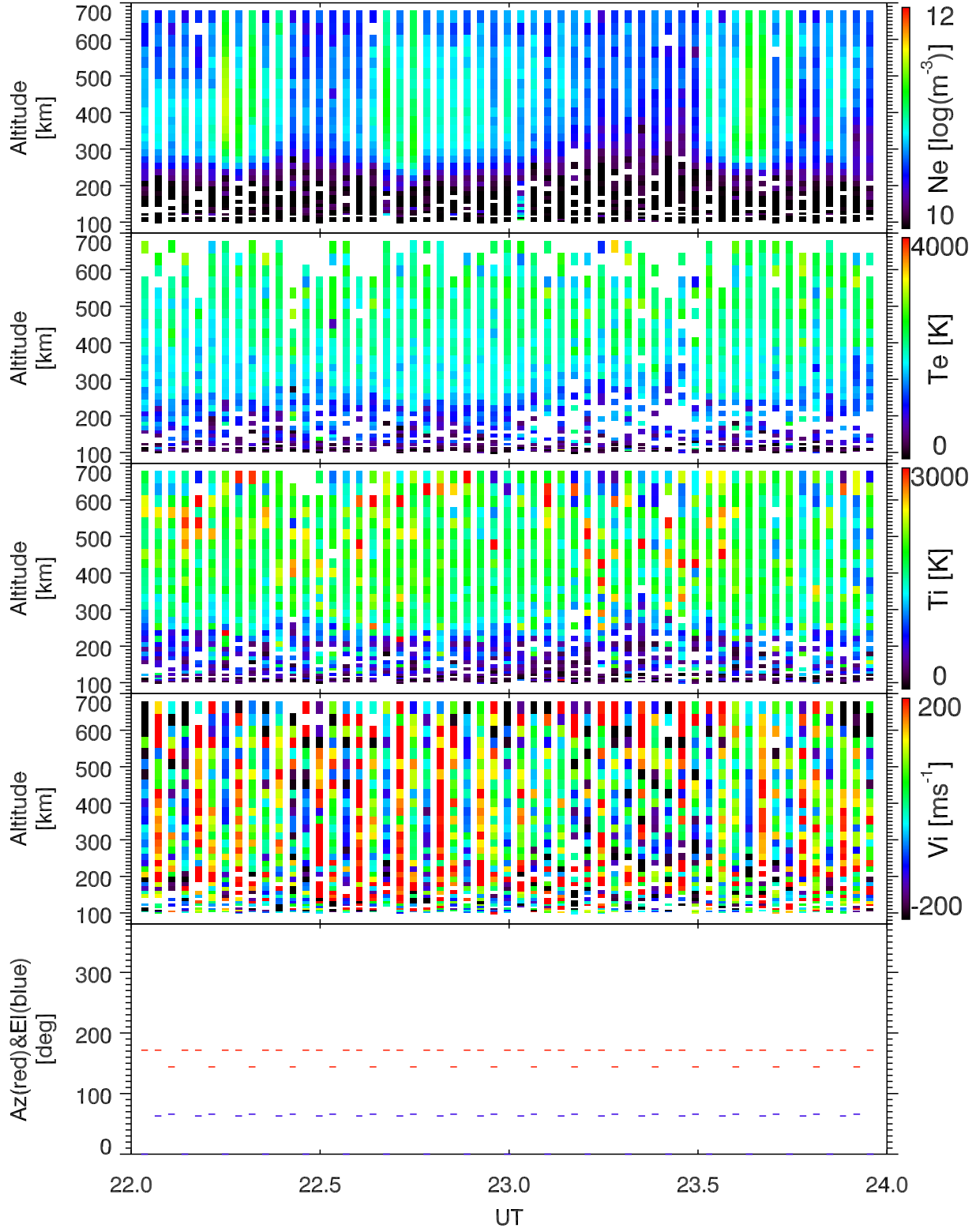
EISCAT 2002-10-07_22_24UT_tau0_ant@32m.
