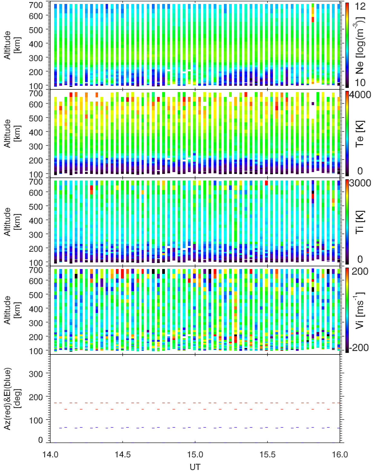
EISCAT 2002-10-08_14_16UT_tau0_ant@32m.
