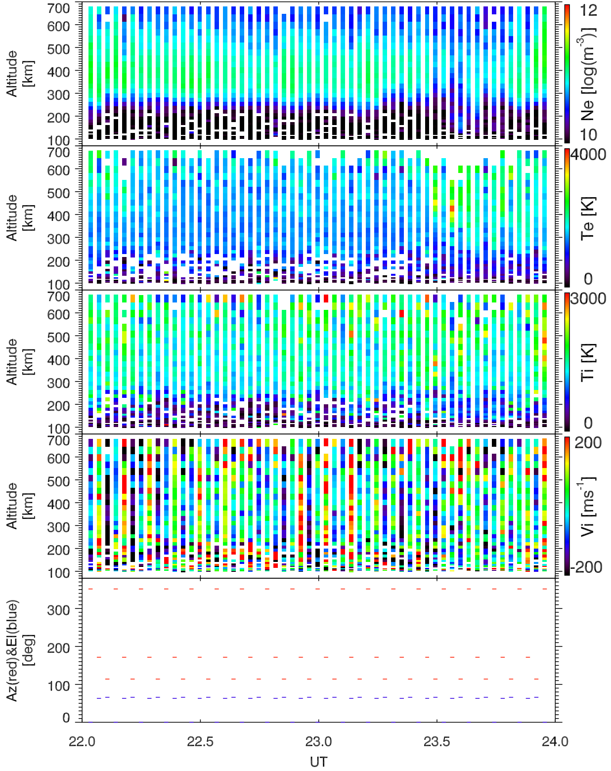
EISCAT 2002-10-08_22_24UT_tau0_ant@32m.
