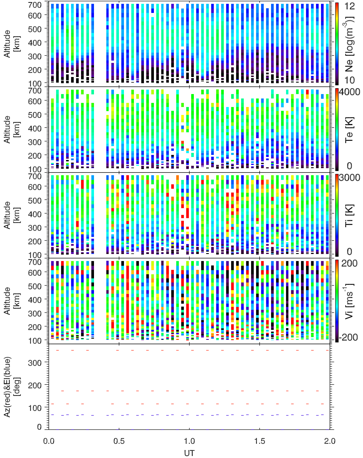
EISCAT 2002-10-09_00_02UT_tau0_ant@32m.
