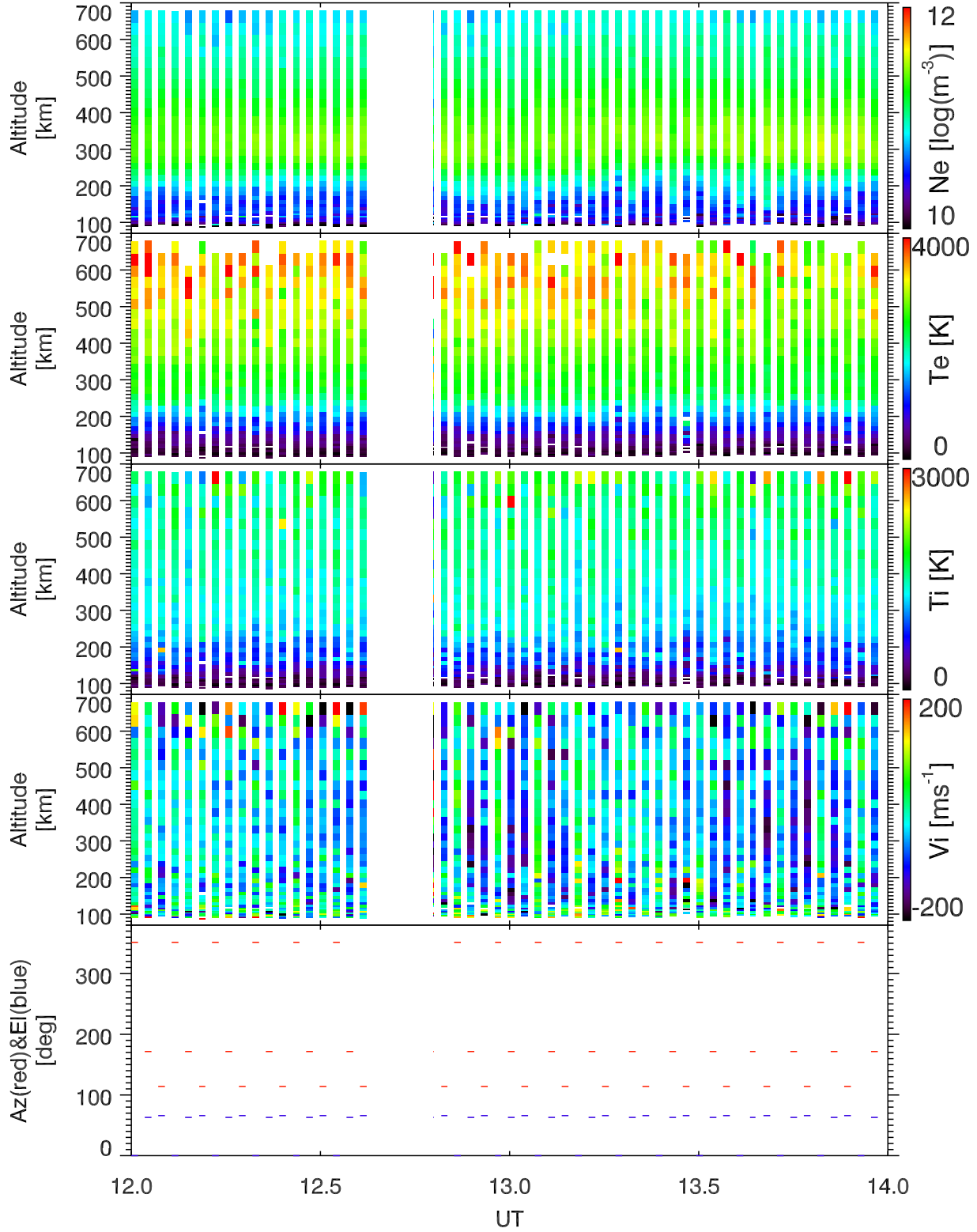
EISCAT 2002-10-09_12_14UT_tau0_ant@32m.
