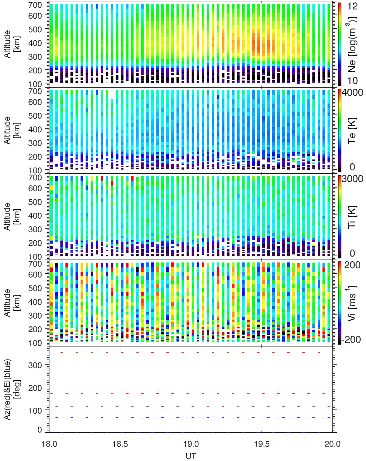
EISCAT 2002-10-09_18_20UT_tau0_ant@32m.
