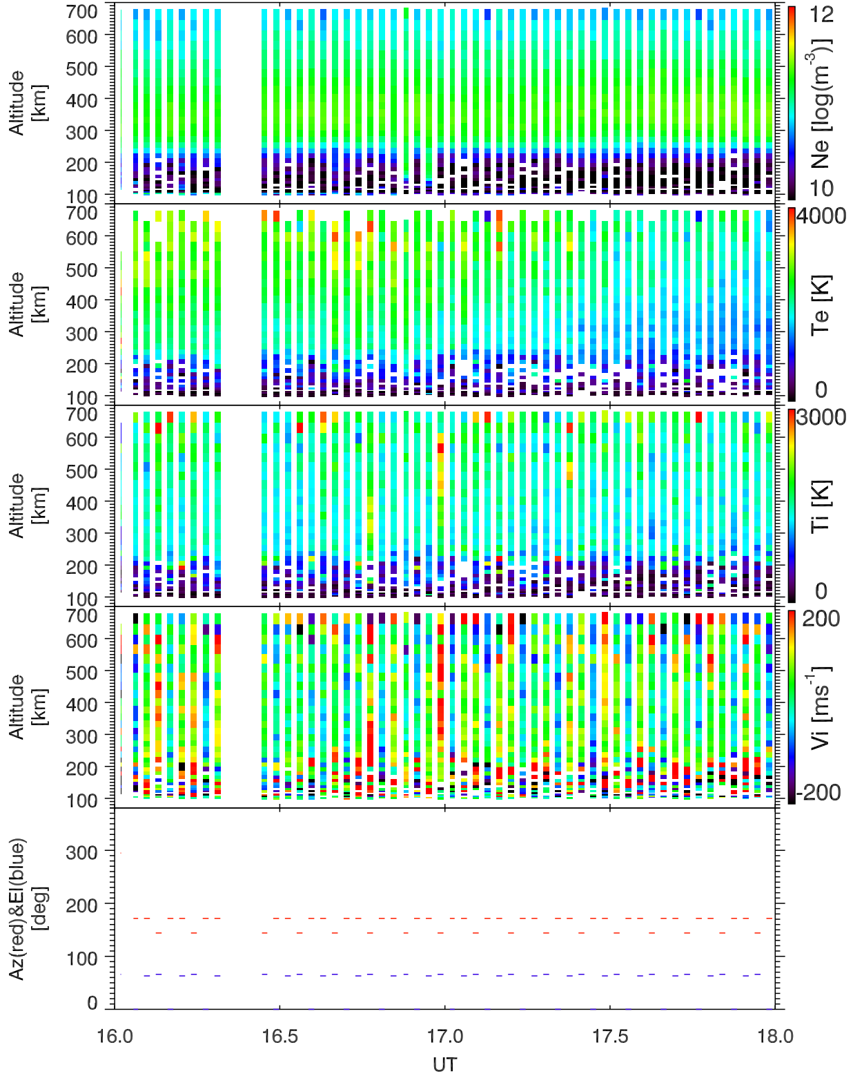
EISCAT 2002-10-10_16_18UT_tau0_ant@32m.
