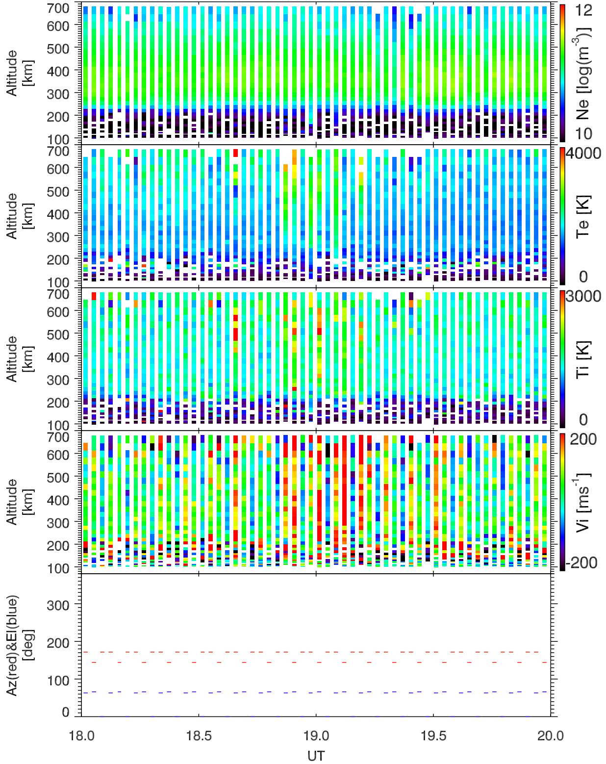
EISCAT 2002-10-10_18_20UT_tau0_ant@32m.
