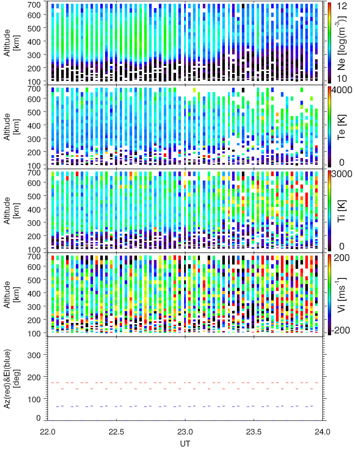
EISCAT 2002-10-10_22_24UT_tau0_ant@32m.
