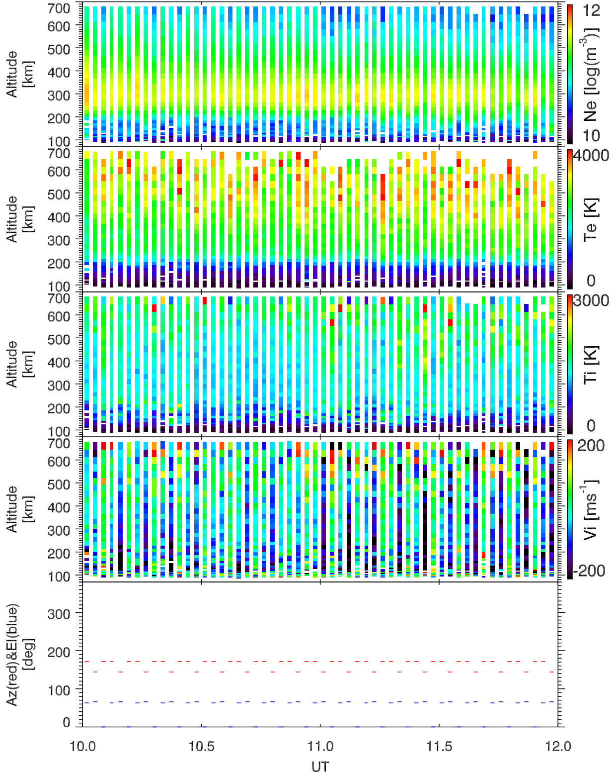
EISCAT 2002-10-11_10_12UT_tau0_ant@32m.
