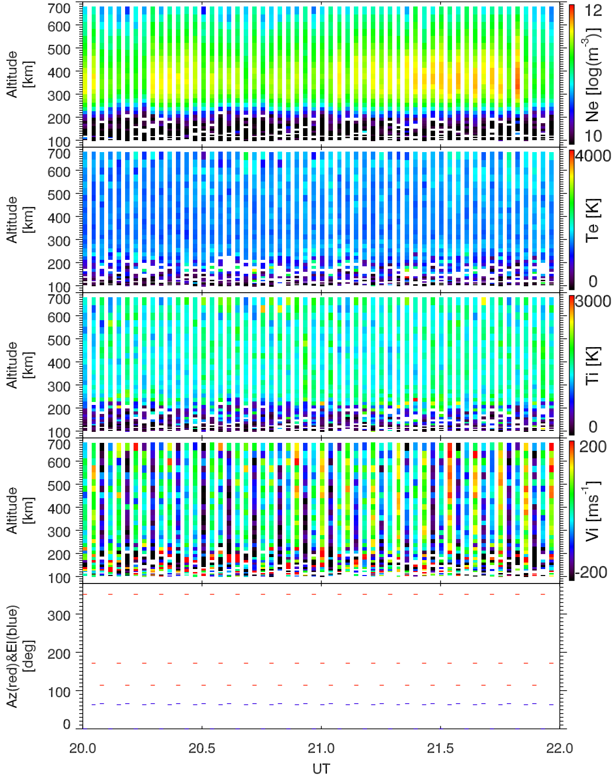
EISCAT 2002-10-11_20_22UT_tau0_ant@32m.
